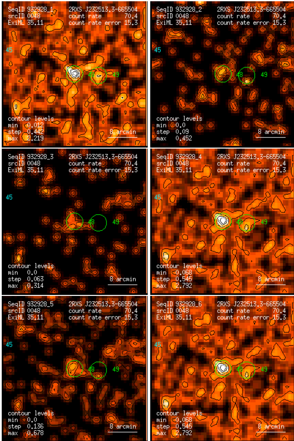
Figure 48: RASS 932928: detection 0048: band rate images, Gaussian filter: (1) PSPC channels 11 – 41, (2) 52 – 90, (3) 91 – 201, (4) 11 – 235, (5) 52 – 201, (6) 11 – 201. Broad band rates in counts/ks. Band rate contour levels in counts/ks/arcmin 2 .
