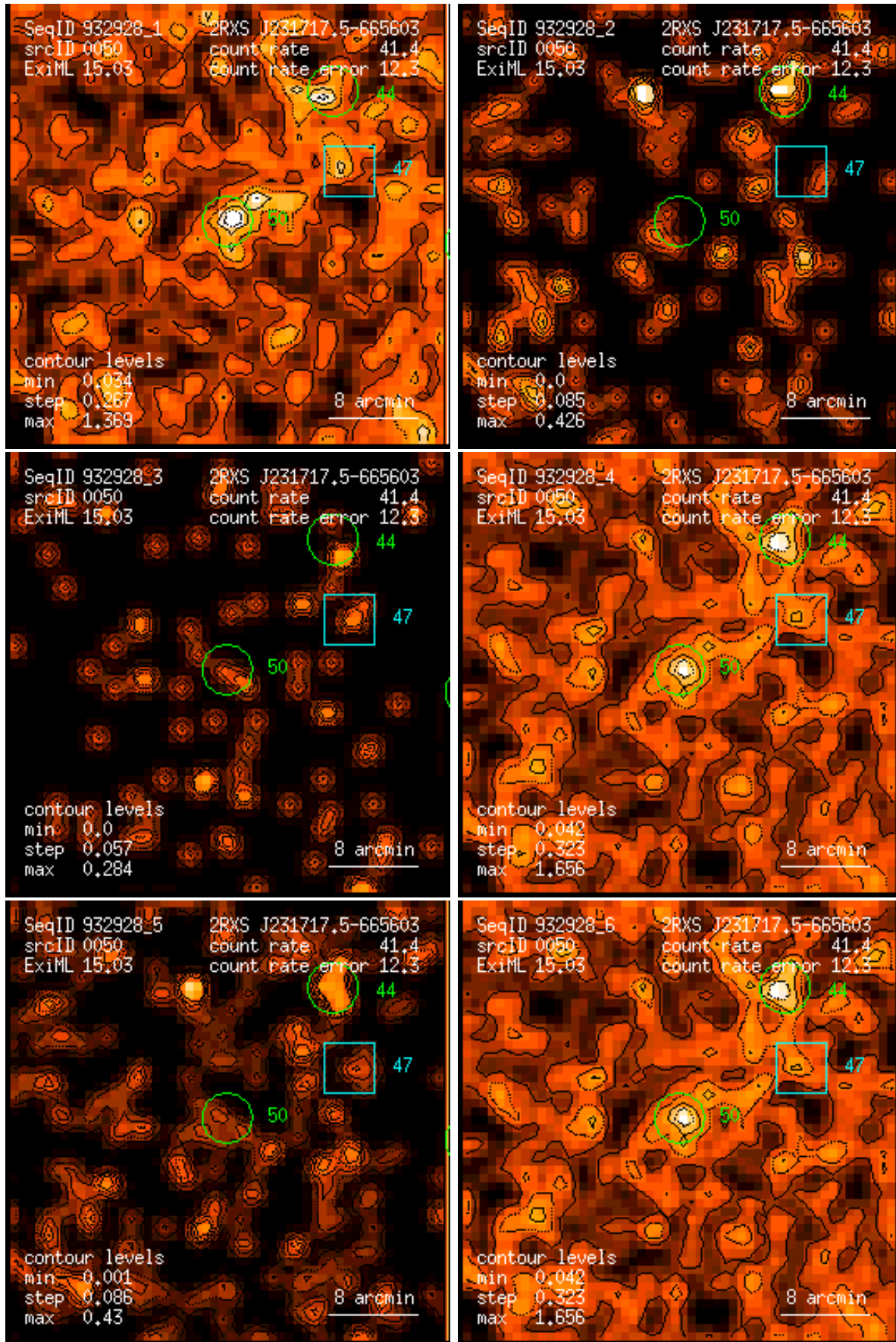
Figure 50: RASS 932928: detection 0050: band rate images, Gaussian filter: (1) PSPC channels 11 – 41, (2) 52 – 90, (3) 91 – 201, (4) 11 – 235, (5) 52 – 201, (6) 11 – 201. Broad band rates in counts/ks. Band rate contour levels in counts/ks/arcmin 2 .
