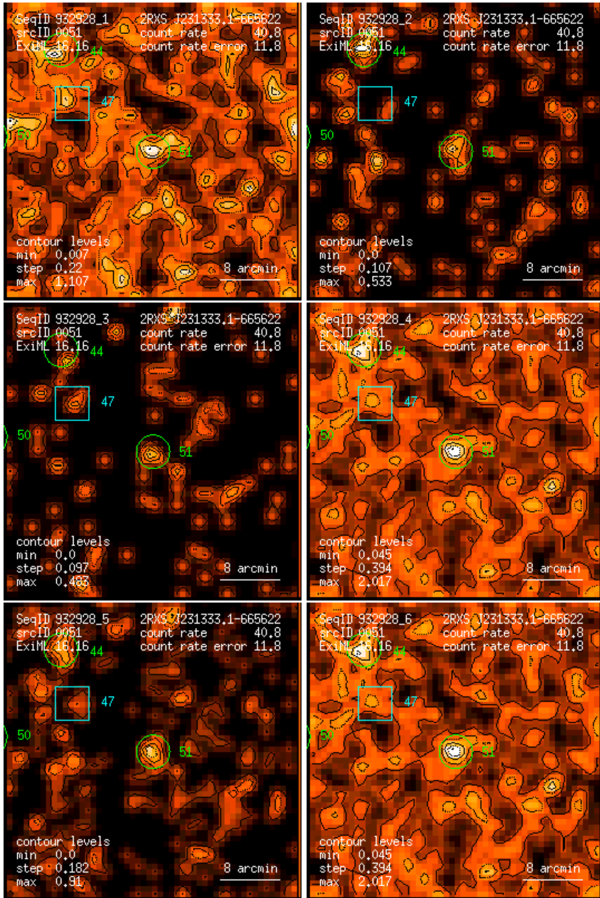
Figure 51: RASS 932928: detection 0051: band rate images, Gaussian filter: (1) PSPC channels 11 – 41, (2) 52 – 90, (3) 91 – 201, (4) 11 – 235, (5) 52 – 201, (6) 11 – 201. Broad band rates in counts/ks. Band rate contour levels in counts/ks/arcmin 2 .
