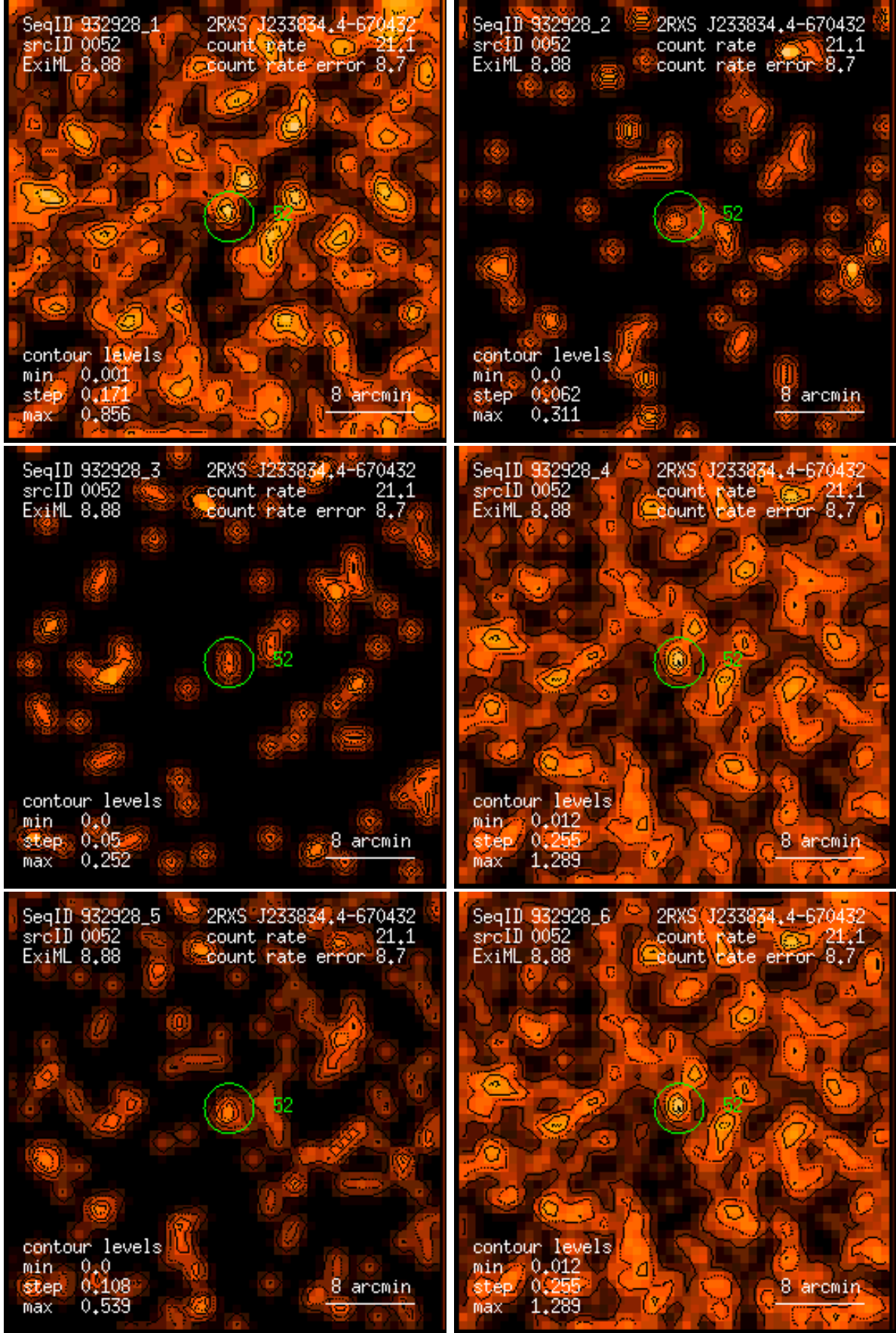
Figure 52: RASS 932928: detection 0052: band rate images, Gaussian filter: (1) PSPC channels 11 – 41, (2) 52 – 90, (3) 91 – 201, (4) 11 – 235, (5) 52 – 201, (6) 11 – 201. Broad band rates in counts/ks. Band rate contour levels in counts/ks/arcmin 2 .
