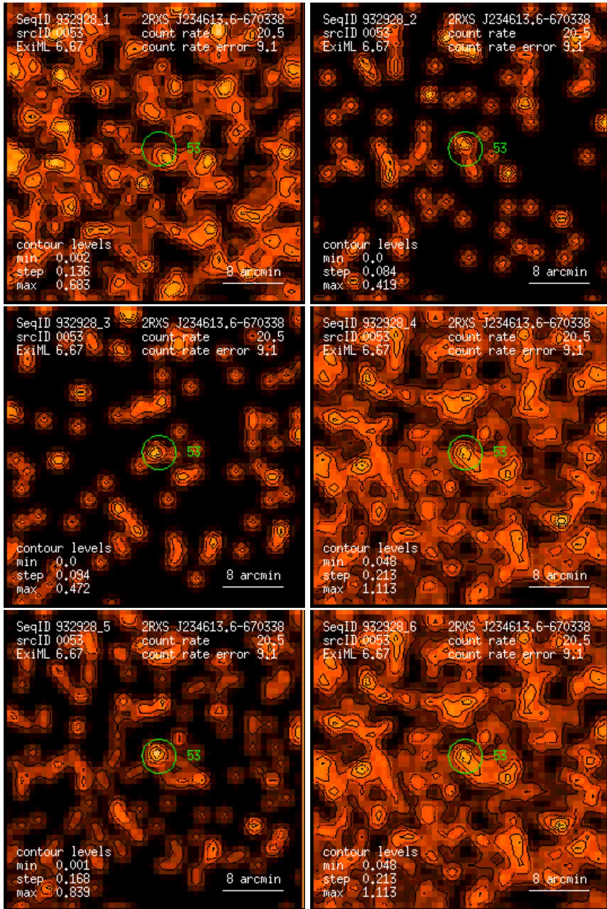
Figure 53: RASS 932928: detection 0053: band rate images, Gaussian filter: (1) PSPC channels 11 – 41, (2) 52 – 90, (3) 91 – 201, (4) 11 – 235, (5) 52 – 201, (6) 11 – 201. Broad band rates in counts/ks. Band rate contour levels in counts/ks/arcmin 2 .
