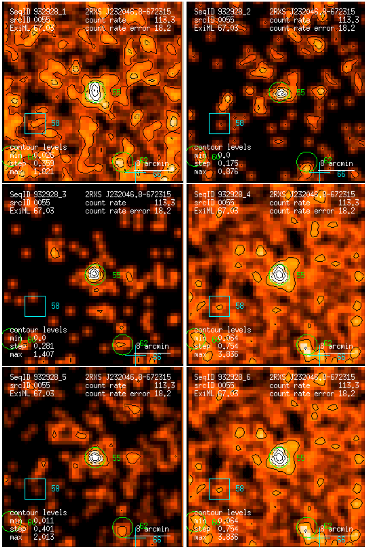
Figure 55: RASS 932928: detection 0055: band rate images, Gaussian filter: (1) PSPC channels 11 – 41, (2) 52 – 90, (3) 91 – 201, (4) 11 – 235, (5) 52 – 201, (6) 11 – 201. Broad band rates in counts/ks. Band rate contour levels in counts/ks/arcmin 2 .
