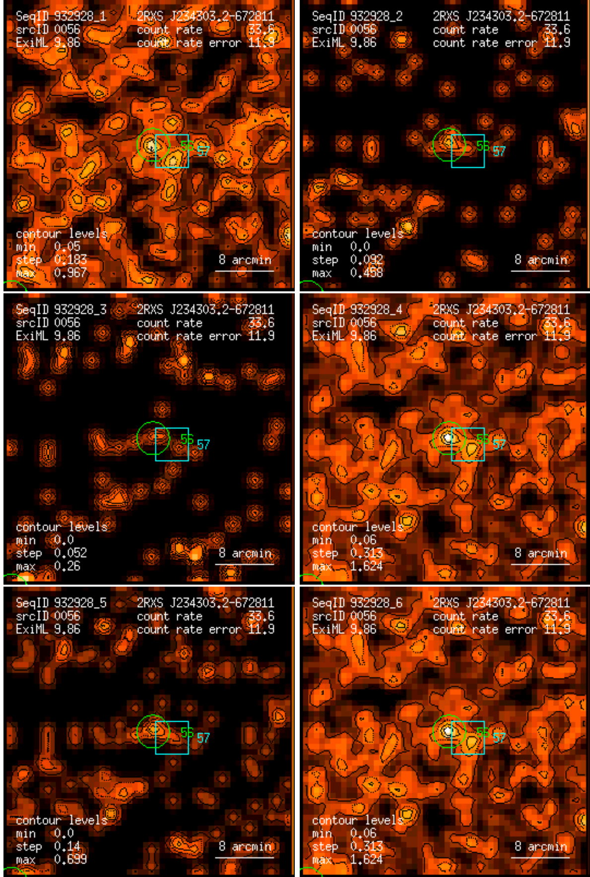
Figure 56: RASS 932928: detection 0056: band rate images, Gaussian filter: (1) PSPC channels 11 – 41, (2) 52 – 90, (3) 91 – 201, (4) 11 – 235, (5) 52 – 201, (6) 11 – 201. Broad band rates in counts/ks. Band rate contour levels in counts/ks/arcmin 2 .
