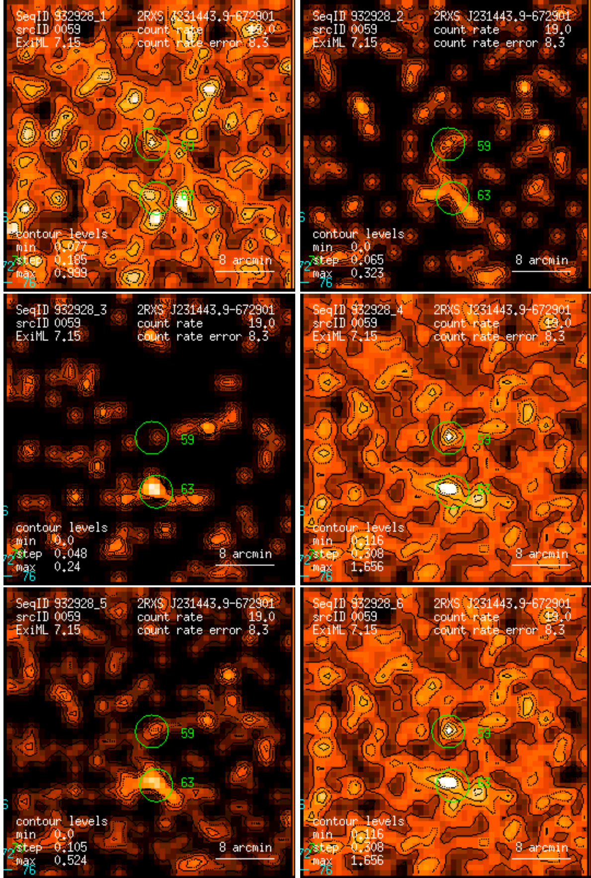
Figure 59: RASS 932928: detection 0059: band rate images, Gaussian filter: (1) PSPC channels 11 – 41, (2) 52 – 90, (3) 91 – 201, (4) 11 – 235, (5) 52 – 201, (6) 11 – 201. Broad band rates in counts/ks. Band rate contour levels in counts/ks/arcmin 2 .
