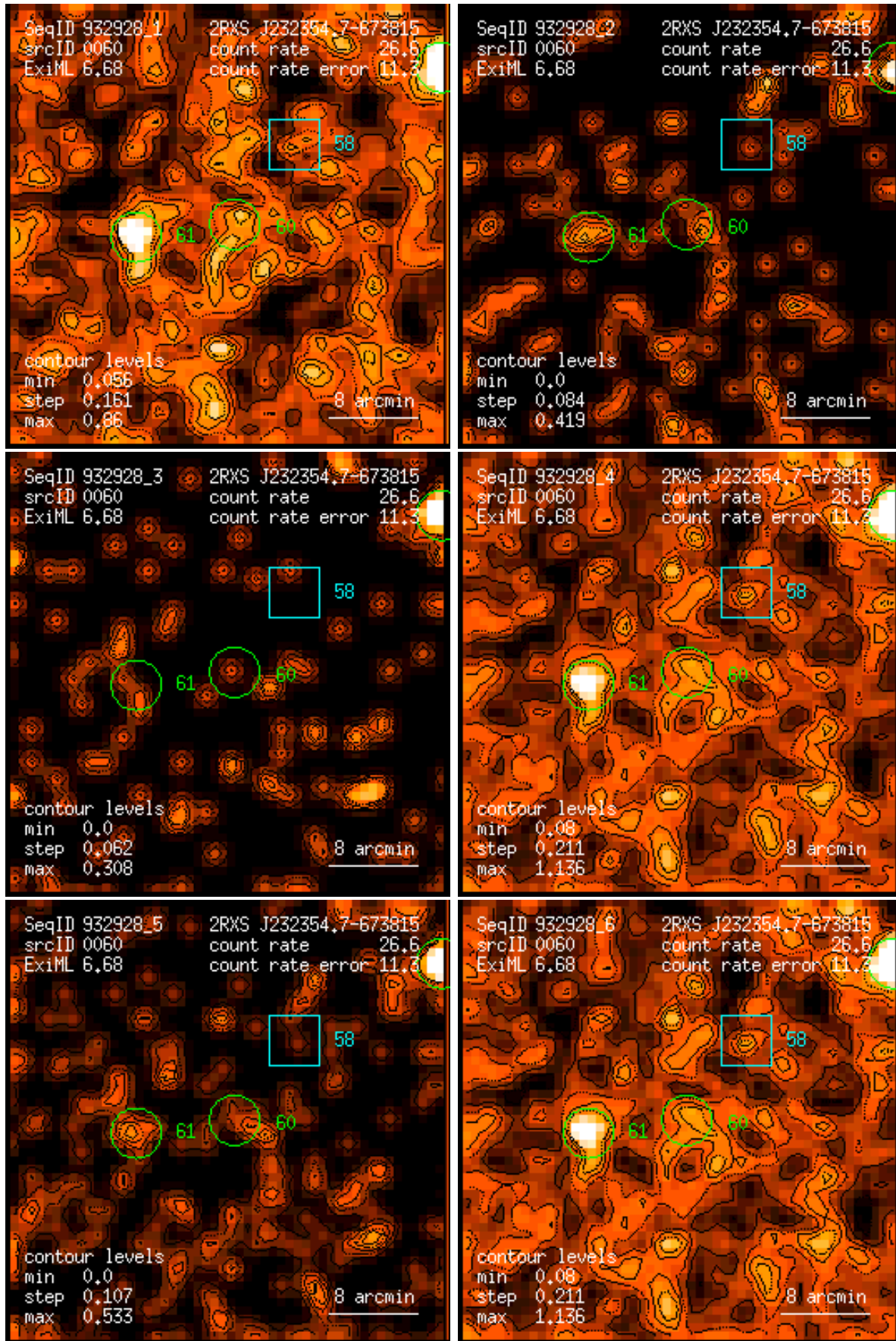
Figure 60: RASS 932928: detection 0060: band rate images, Gaussian filter: (1) PSPC channels 11 – 41, (2) 52 – 90, (3) 91 – 201, (4) 11 – 235, (5) 52 – 201, (6) 11 – 201. Broad band rates in counts/ks. Band rate contour levels in counts/ks/arcmin 2 .
