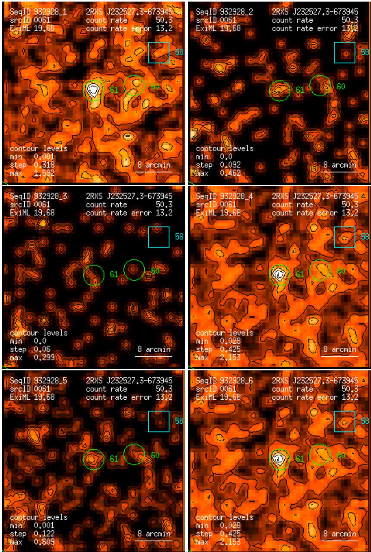
Figure 61: RASS 932928: detection 0061: band rate images, Gaussian filter: (1) PSPC channels 11 – 41, (2) 52 – 90, (3) 91 – 201, (4) 11 – 235, (5) 52 – 201, (6) 11 – 201. Broad band rates in counts/ks. Band rate contour levels in counts/ks/arcmin 2 .
