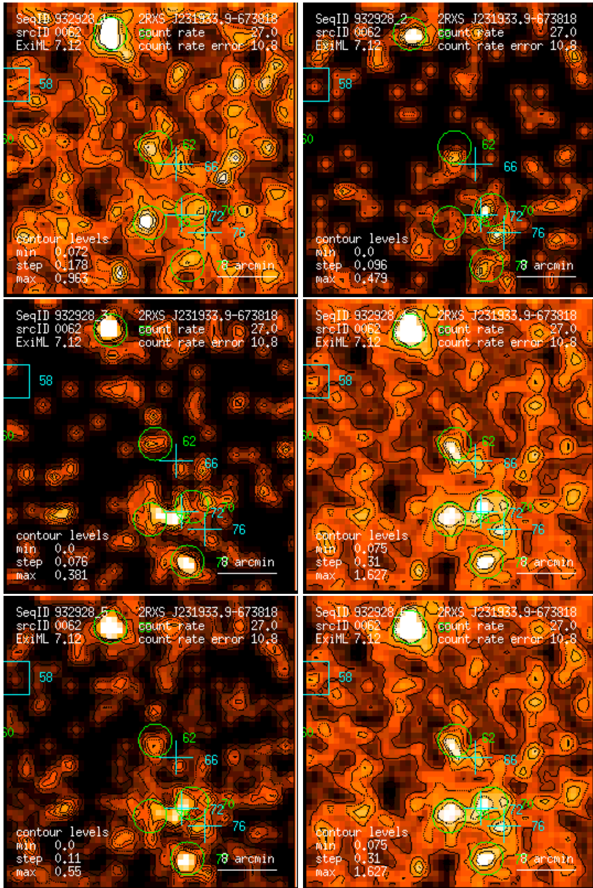
Figure 62: RASS 932928: detection 0062: band rate images, Gaussian filter: (1) PSPC channels 11 – 41, (2) 52 – 90, (3) 91 – 201, (4) 11 – 235, (5) 52 – 201, (6) 11 – 201. Broad band rates in counts/ks. Band rate contour levels in counts/ks/arcmin 2 .
