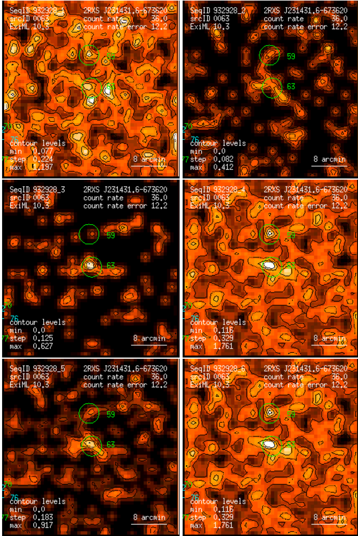
Figure 63: RASS 932928: detection 0063: band rate images, Gaussian filter: (1) PSPC channels 11 – 41, (2) 52 – 90, (3) 91 – 201, (4) 11 – 235, (5) 52 – 201, (6) 11 – 201. Broad band rates in counts/ks. Band rate contour levels in counts/ks/arcmin 2 .
