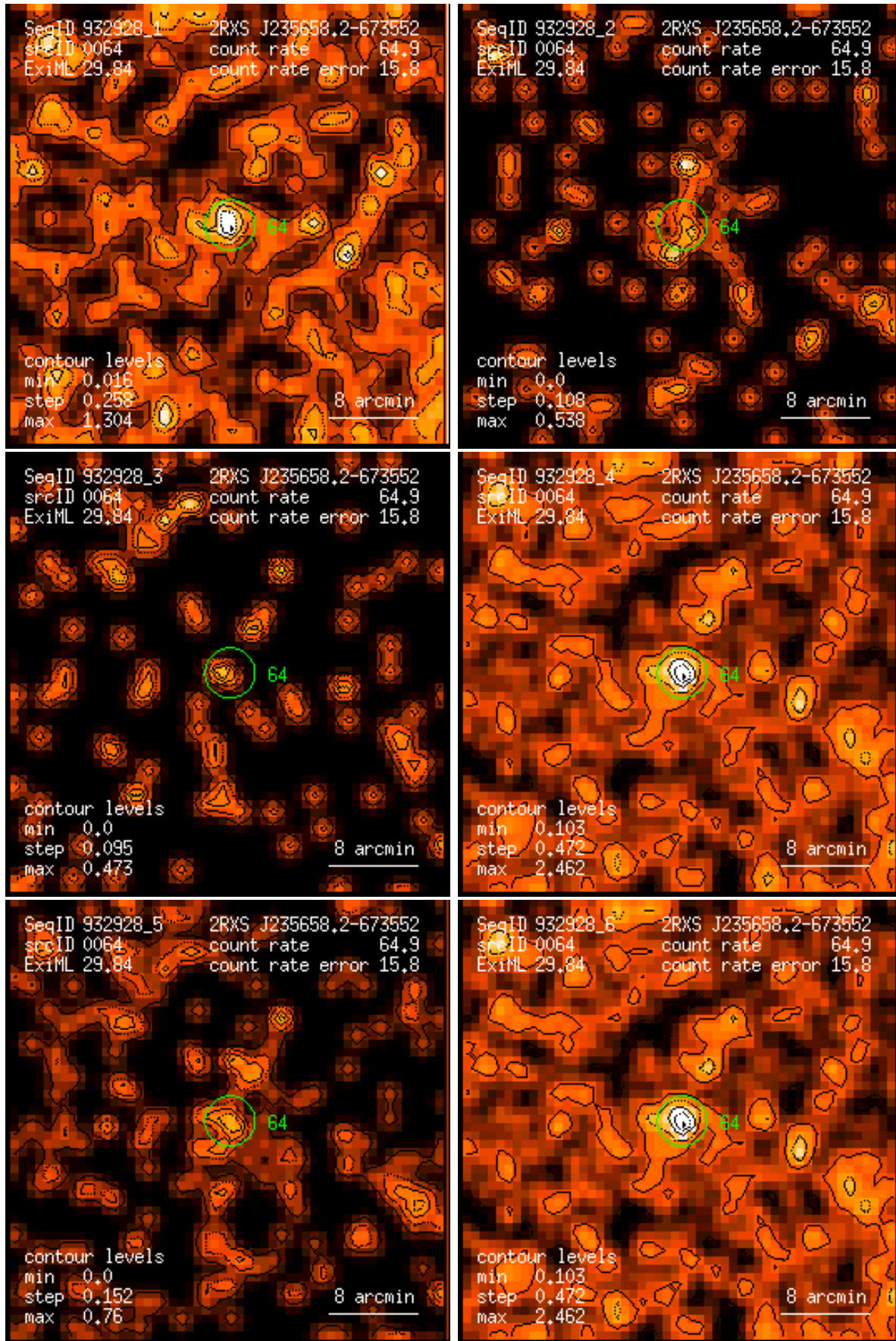
Figure 64: RASS 932928: detection 0064: band rate images, Gaussian filter: (1) PSPC channels 11 – 41, (2) 52 – 90, (3) 91 – 201, (4) 11 – 235, (5) 52 – 201, (6) 11 – 201. Broad band rates in counts/ks. Band rate contour levels in counts/ks/arcmin 2 .
