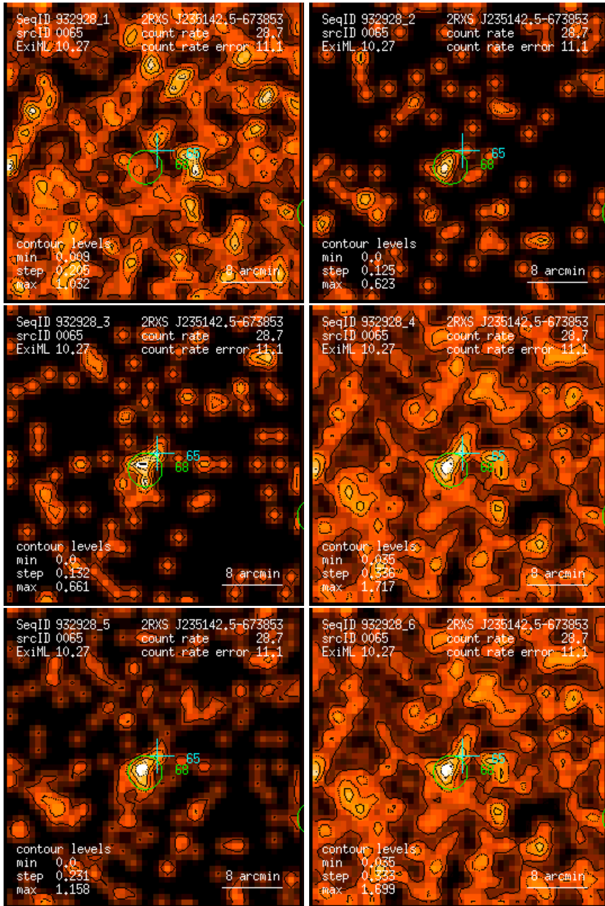
Figure 65: RASS 932928: detection 0065: band rate images, Gaussian filter: (1) PSPC channels 11 – 41, (2) 52 – 90, (3) 91 – 201, (4) 11 – 235, (5) 52 – 201, (6) 11 – 201. Broad band rates in counts/ks. Band rate contour levels in counts/ks/arcmin 2 .
