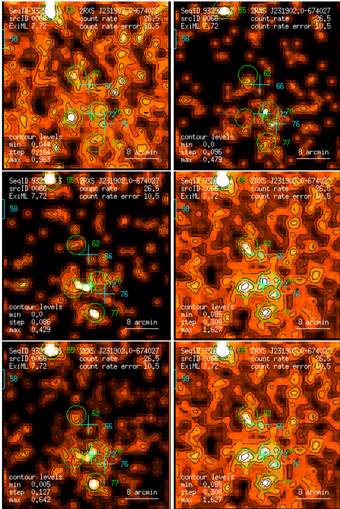
Figure 66: RASS 932928: detection 0066: band rate images, Gaussian filter: (1) PSPC channels 11 – 41, (2) 52 – 90, (3) 91 – 201, (4) 11 – 235, (5) 52 – 201, (6) 11 – 201. Broad band rates in counts/ks. Band rate contour levels in counts/ks/arcmin 2 .
