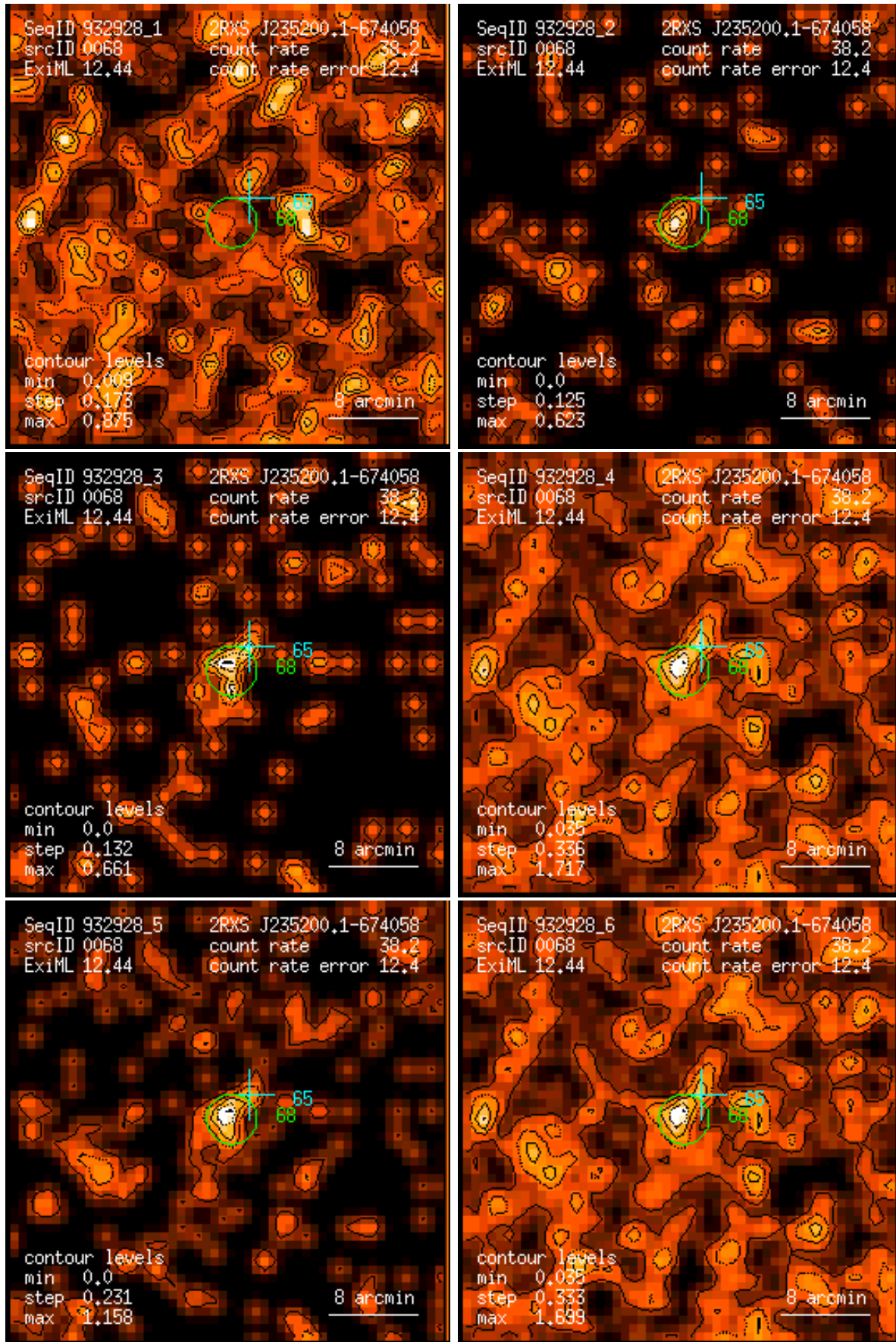
Figure 68: RASS 932928: detection 0068: band rate images, Gaussian filter: (1) PSPC channels 11 – 41, (2) 52 – 90, (3) 91 – 201, (4) 11 – 235, (5) 52 – 201, (6) 11 – 201. Broad band rates in counts/ks. Band rate contour levels in counts/ks/arcmin 2 .
