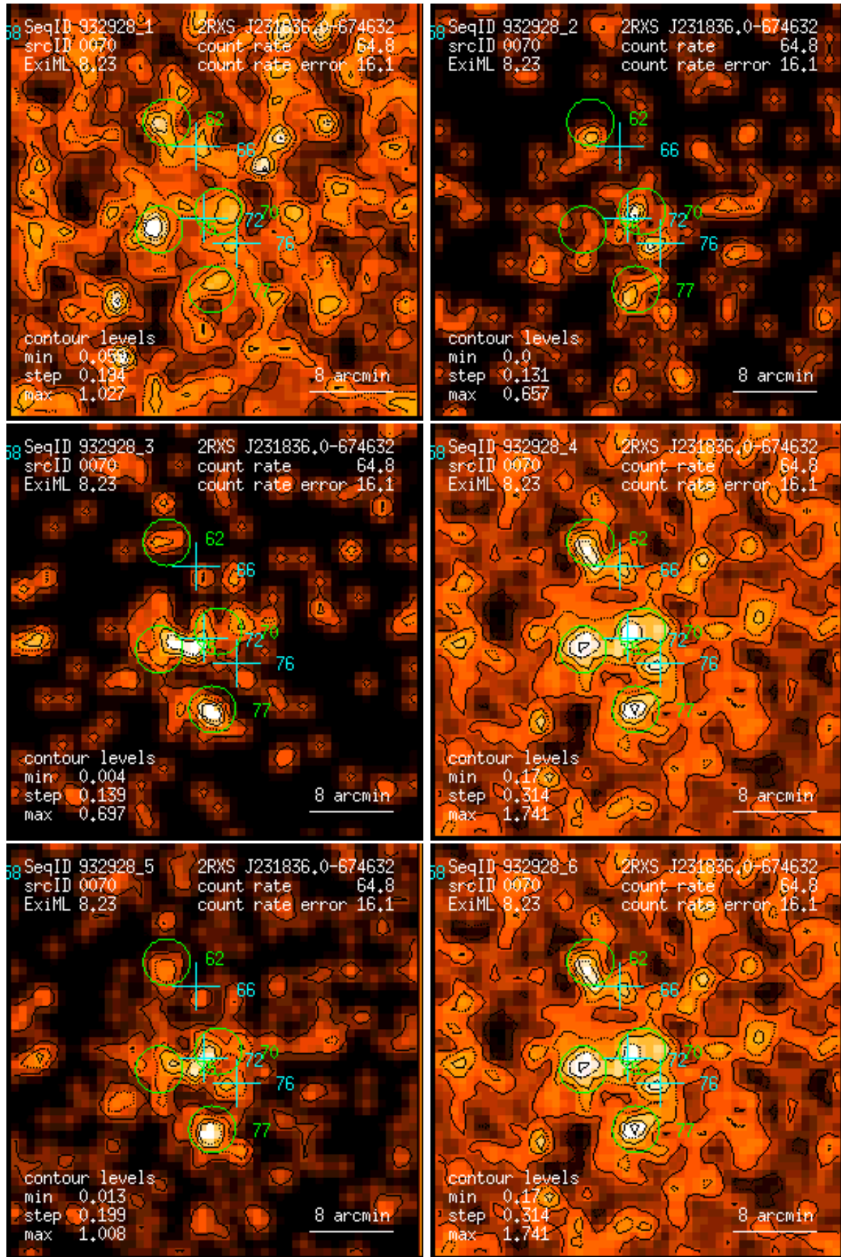
Figure 70: RASS 932928: detection 0070: band rate images, Gaussian filter: (1) PSPC channels 11 – 41, (2) 52 – 90, (3) 91 – 201, (4) 11 – 235, (5) 52 – 201, (6) 11 – 201. Broad band rates in counts/ks. Band rate contour levels in counts/ks/arcmin 2 .
