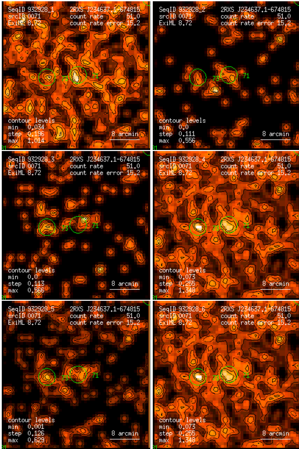
Figure 71: RASS 932928: detection 0071: band rate images, Gaussian filter: (1) PSPC channels 11 – 41, (2) 52 – 90, (3) 91 – 201, (4) 11 – 235, (5) 52 – 201, (6) 11 – 201. Broad band rates in counts/ks. Band rate contour levels in counts/ks/arcmin 2 .
