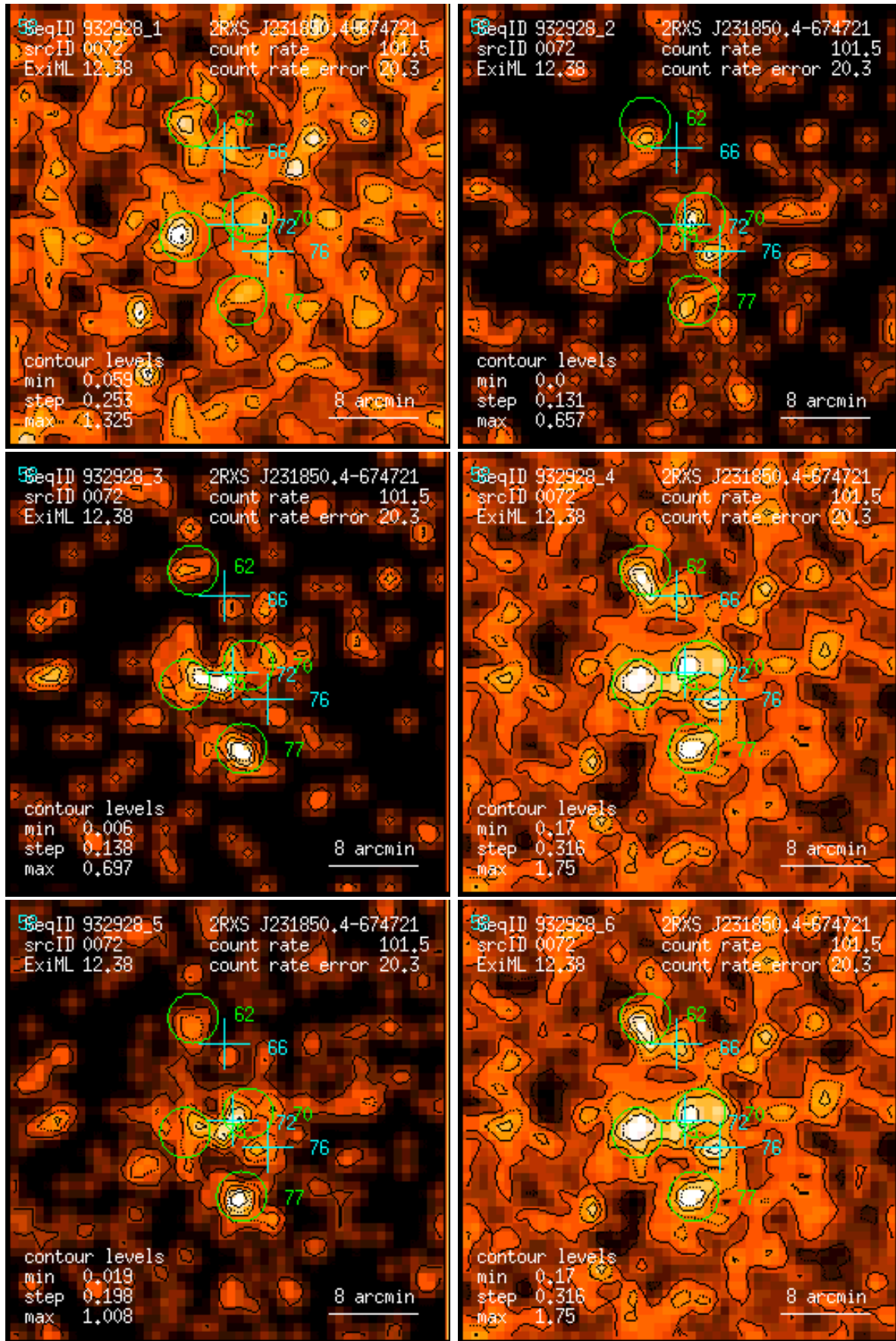
Figure 72: RASS 932928: detection 0072: band rate images, Gaussian filter: (1) PSPC channels 11 – 41, (2) 52 – 90, (3) 91 – 201, (4) 11 – 235, (5) 52 – 201, (6) 11 – 201. Broad band rates in counts/ks. Band rate contour levels in counts/ks/arcmin 2 .
