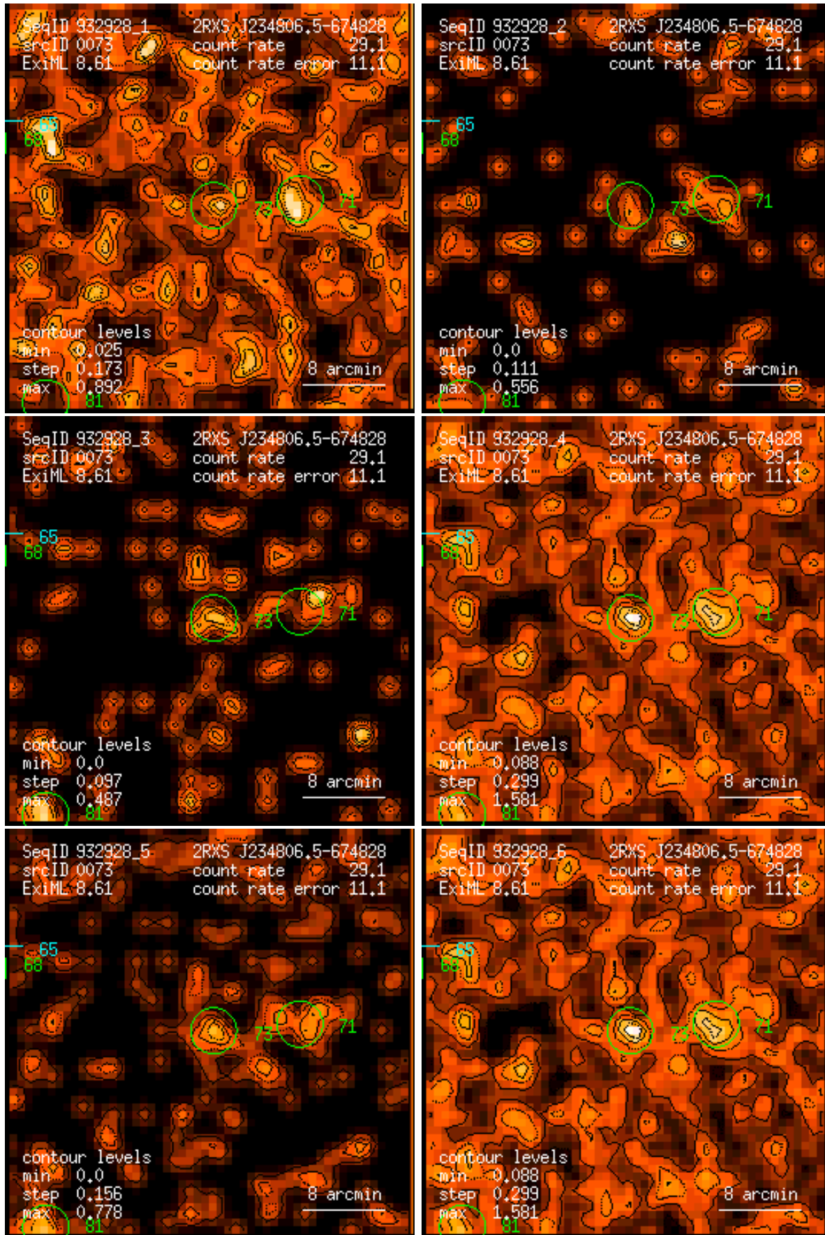
Figure 73: RASS 932928: detection 0073: band rate images, Gaussian filter: (1) PSPC channels 11 – 41, (2) 52 – 90, (3) 91 – 201, (4) 11 – 235, (5) 52 – 201, (6) 11 – 201. Broad band rates in counts/ks. Band rate contour levels in counts/ks/arcmin 2 .
