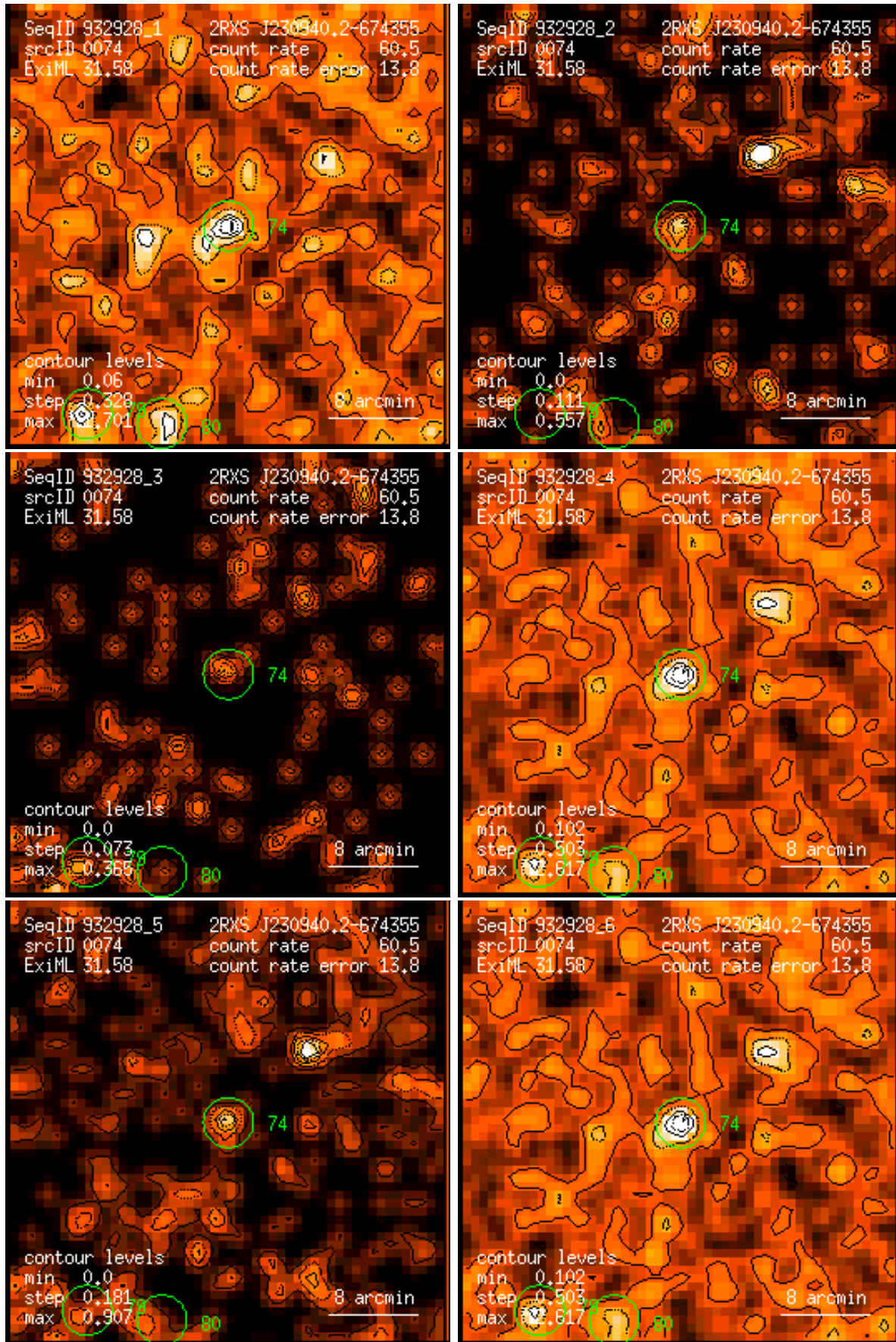
Figure 74: RASS 932928: detection 0074: band rate images, Gaussian filter: (1) PSPC channels 11 – 41, (2) 52 – 90, (3) 91 – 201, (4) 11 – 235, (5) 52 – 201, (6) 11 – 201. Broad band rates in counts/ks. Band rate contour levels in counts/ks/arcmin 2 .
