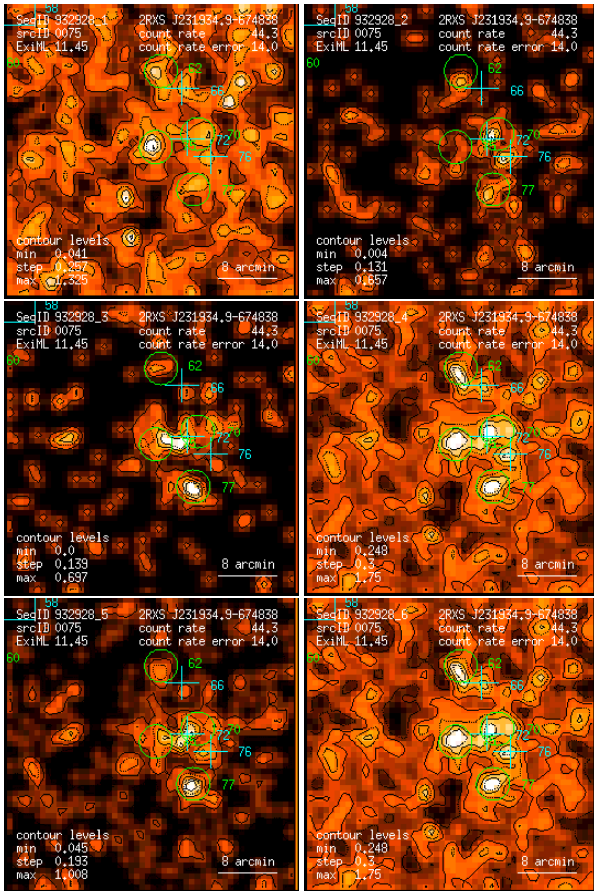
Figure 75: RASS 932928: detection 0075: band rate images, Gaussian filter: (1) PSPC channels 11 – 41, (2) 52 – 90, (3) 91 – 201, (4) 11 – 235, (5) 52 – 201, (6) 11 – 201. Broad band rates in counts/ks. Band rate contour levels in counts/ks/arcmin 2 .
