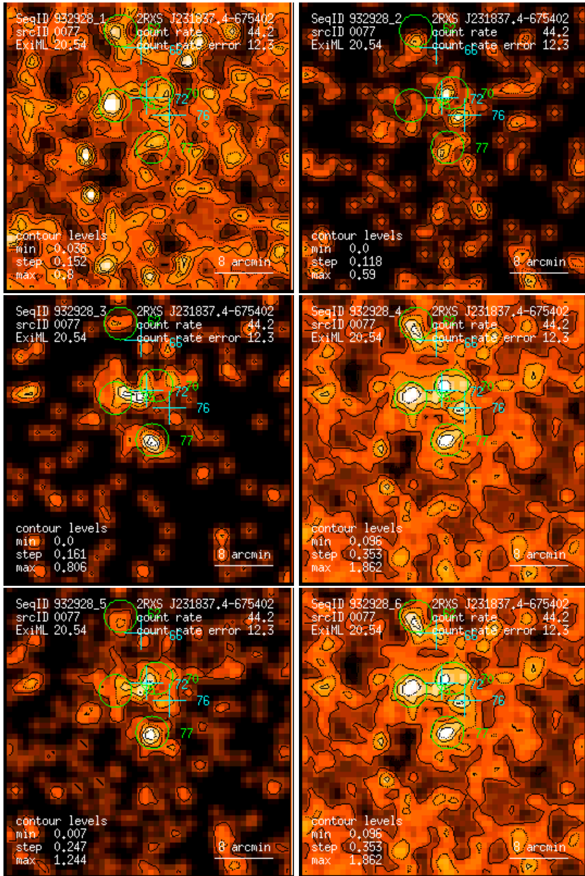
Figure 77: RASS 932928: detection 0077: band rate images, Gaussian filter: (1) PSPC channels 11 – 41, (2) 52 – 90, (3) 91 – 201, (4) 11 – 235, (5) 52 – 201, (6) 11 – 201. Broad band rates in counts/ks. Band rate contour levels in counts/ks/arcmin 2 .
