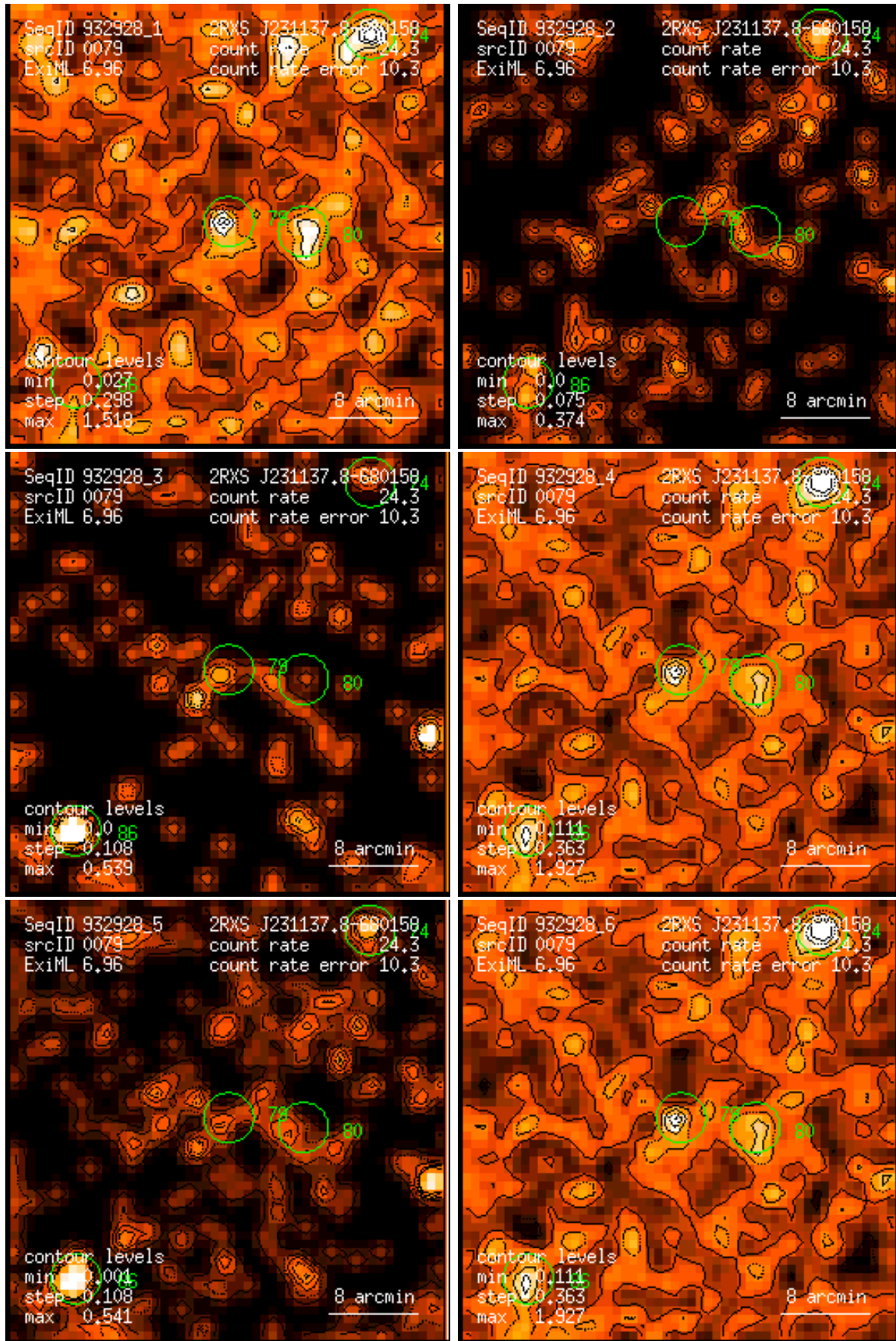
Figure 79: RASS 932928: detection 0079: band rate images, Gaussian filter: (1) PSPC channels 11 – 41, (2) 52 – 90, (3) 91 – 201, (4) 11 – 235, (5) 52 – 201, (6) 11 – 201. Broad band rates in counts/ks. Band rate contour levels in counts/ks/arcmin 2 .
