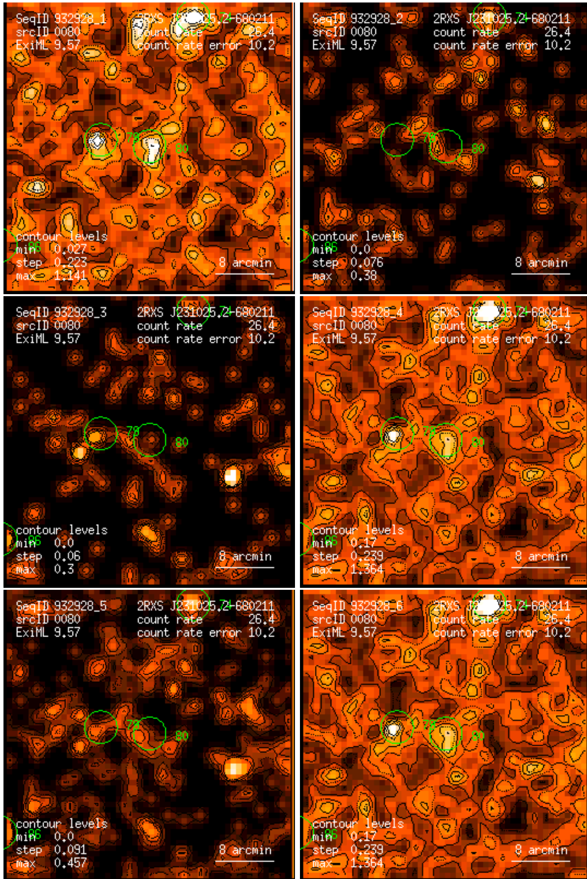
Figure 80: RASS 932928: detection 0080: band rate images, Gaussian filter: (1) PSPC channels 11 – 41, (2) 52 – 90, (3) 91 – 201, (4) 11 – 235, (5) 52 – 201, (6) 11 – 201. Broad band rates in counts/ks. Band rate contour levels in counts/ks/arcmin 2 .
