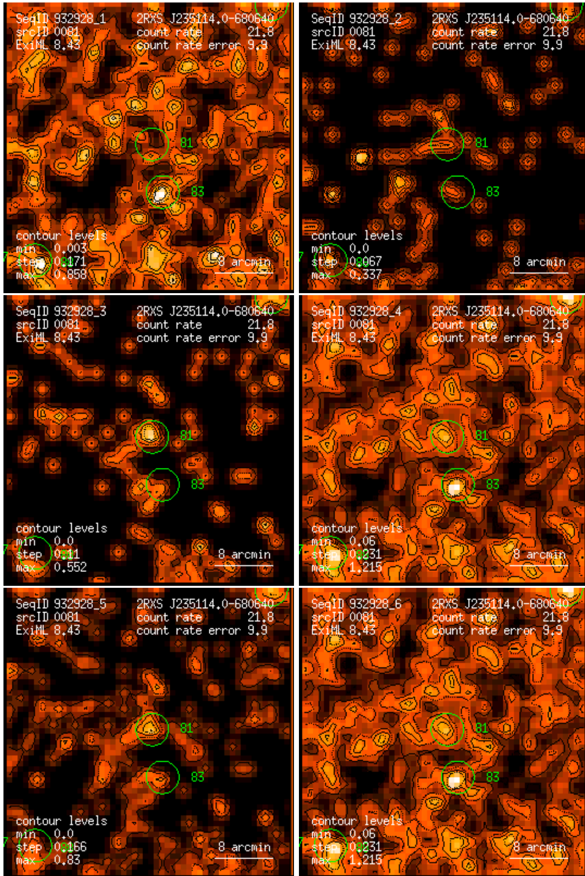
Figure 81: RASS 932928: detection 0081: band rate images, Gaussian filter: (1) PSPC channels 11 – 41, (2) 52 – 90, (3) 91 – 201, (4) 11 – 235, (5) 52 – 201, (6) 11 – 201. Broad band rates in counts/ks. Band rate contour levels in counts/ks/arcmin 2 .
