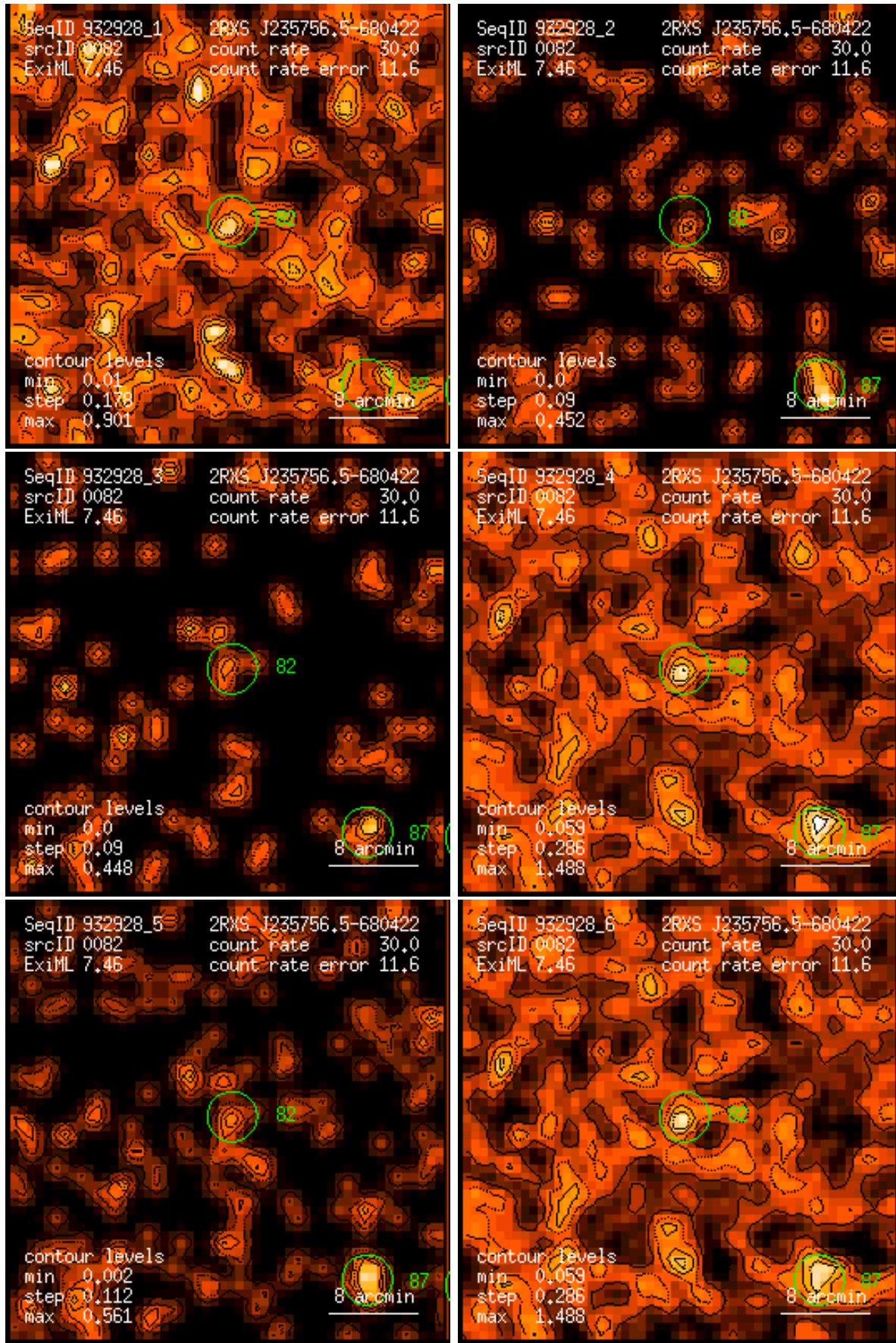
Figure 82: RASS 932928: detection 0082: band rate images, Gaussian filter: (1) PSPC channels 11 – 41, (2) 52 – 90, (3) 91 – 201, (4) 11 – 235, (5) 52 – 201, (6) 11 – 201. Broad band rates in counts/ks. Band rate contour levels in counts/ks/arcmin 2 .
