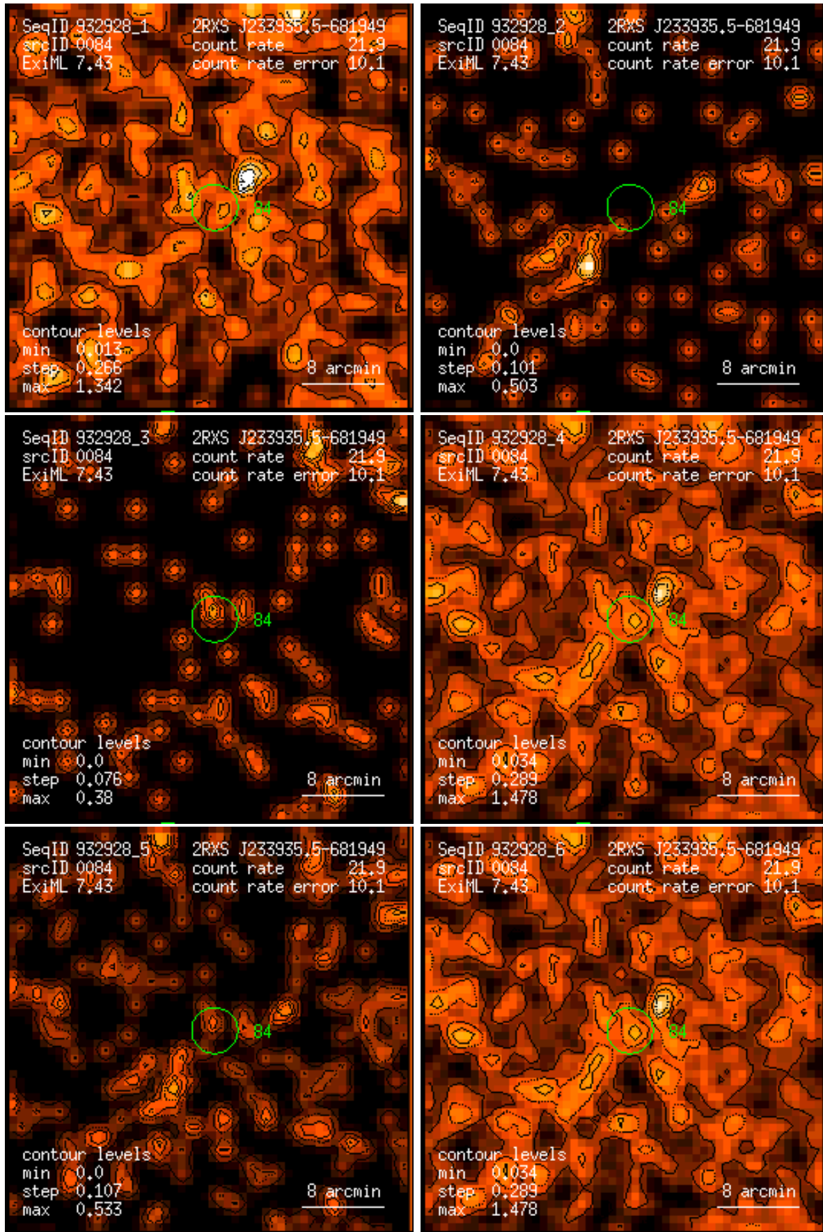
Figure 84: RASS 932928: detection 0084: band rate images, Gaussian filter: (1) PSPC channels 11 – 41, (2) 52 – 90, (3) 91 – 201, (4) 11 – 235, (5) 52 – 201, (6) 11 – 201. Broad band rates in counts/ks. Band rate contour levels in counts/ks/arcmin 2 .
