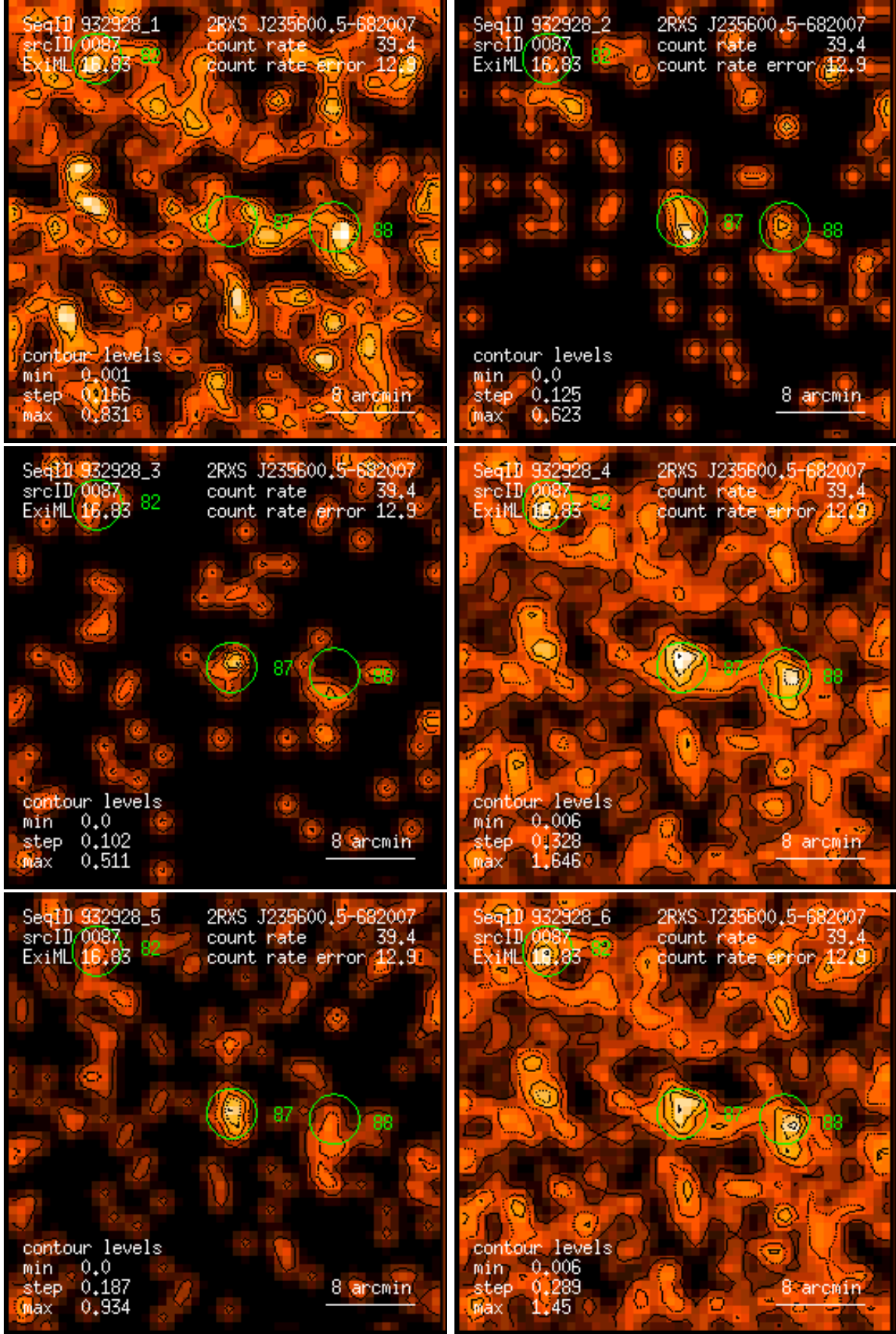
Figure 87: RASS 932928: detection 0087: band rate images, Gaussian filter: (1) PSPC channels 11 – 41, (2) 52 – 90, (3) 91 – 201, (4) 11 – 235, (5) 52 – 201, (6) 11 – 201. Broad band rates in counts/ks. Band rate contour levels in counts/ks/arcmin 2 .
