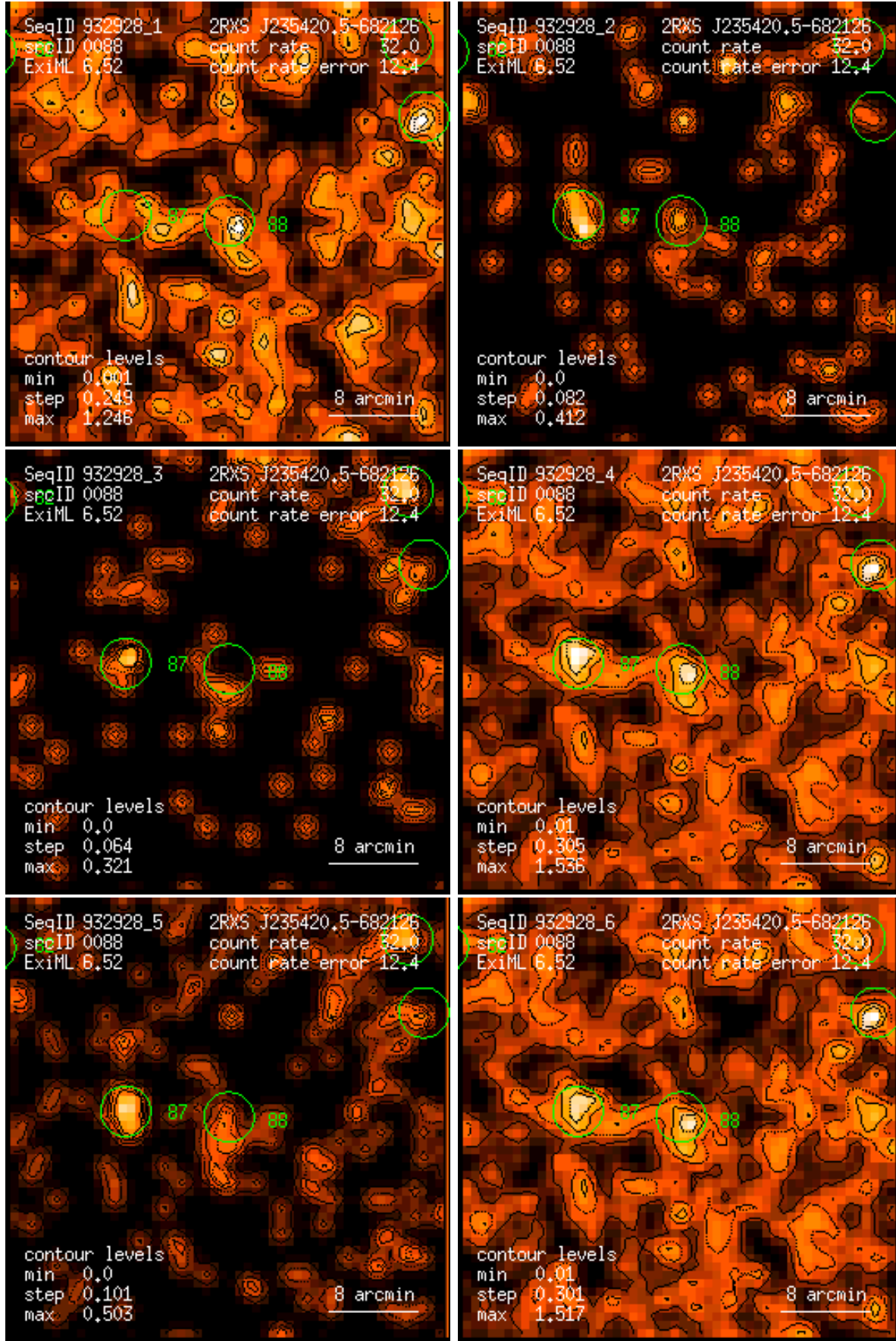
Figure 88: RASS 932928: detection 0088: band rate images, Gaussian filter: (1) PSPC channels 11 – 41, (2) 52 – 90, (3) 91 – 201, (4) 11 – 235, (5) 52 – 201, (6) 11 – 201. Broad band rates in counts/ks. Band rate contour levels in counts/ks/arcmin 2 .
