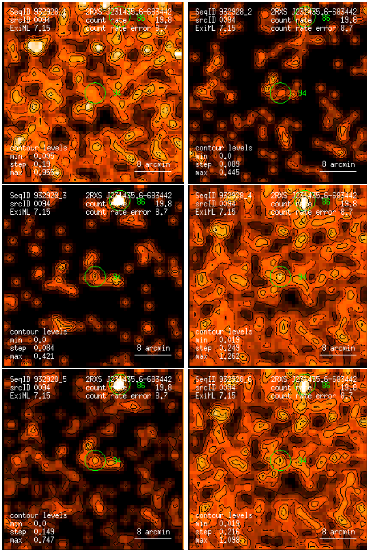
Figure 94: RASS 932928: detection 0094: band rate images, Gaussian filter: (1) PSPC channels 11 – 41, (2) 52 – 90, (3) 91 – 201, (4) 11 – 235, (5) 52 – 201, (6) 11 – 201. Broad band rates in counts/ks. Band rate contour levels in counts/ks/arcmin 2 .
