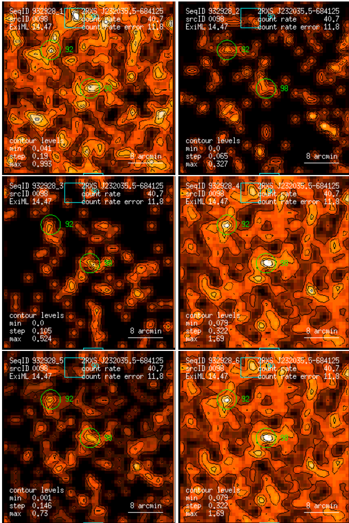
Figure 98: RASS 932928: detection 0098: band rate images, Gaussian filter: (1) PSPC channels 11 – 41, (2) 52 – 90, (3) 91 – 201, (4) 11 – 235, (5) 52 – 201, (6) 11 – 201. Broad band rates in counts/ks. Band rate contour levels in counts/ks/arcmin 2 .
