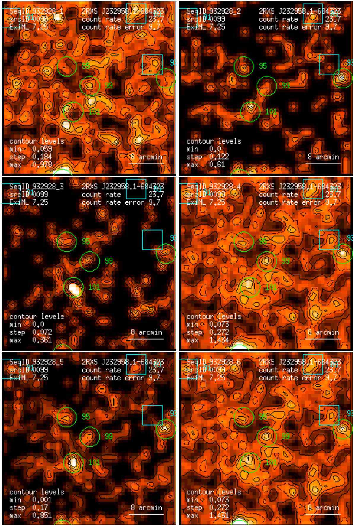
Figure 99: RASS 932928: detection 0099: band rate images, Gaussian filter: (1) PSPC channels 11 – 41, (2) 52 – 90, (3) 91 – 201, (4) 11 – 235, (5) 52 – 201, (6) 11 – 201. Broad band rates in counts/ks. Band rate contour levels in counts/ks/arcmin 2 .
