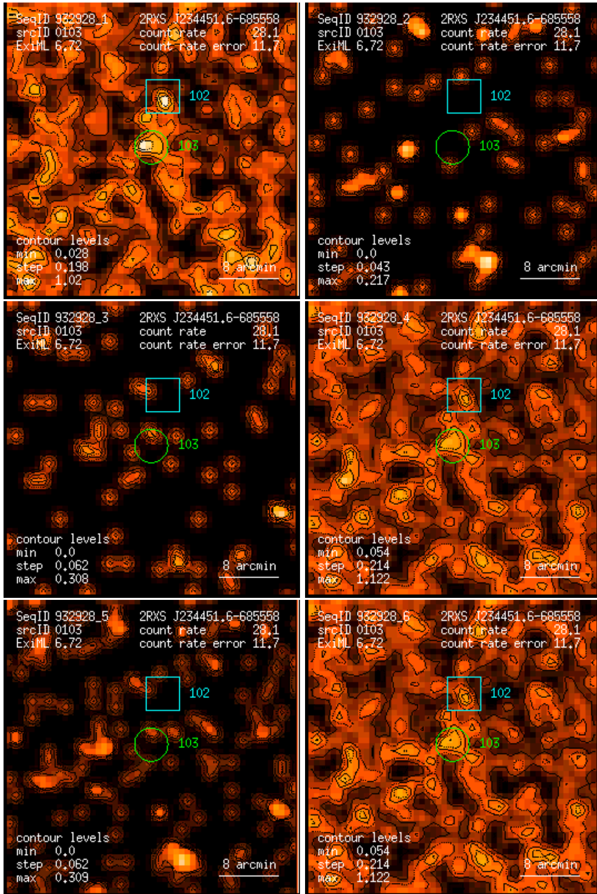
Figure 103: RASS 932928: detection 0103: band rate images, Gaussian filter: (1) PSPC channels 11 – 41, (2) 52 – 90, (3) 91 – 201, (4) 11 – 235, (5) 52 – 201, (6) 11 – 201. Broad band rates in counts/ks. Band rate contour levels in counts/ks/arcmin 2 .
