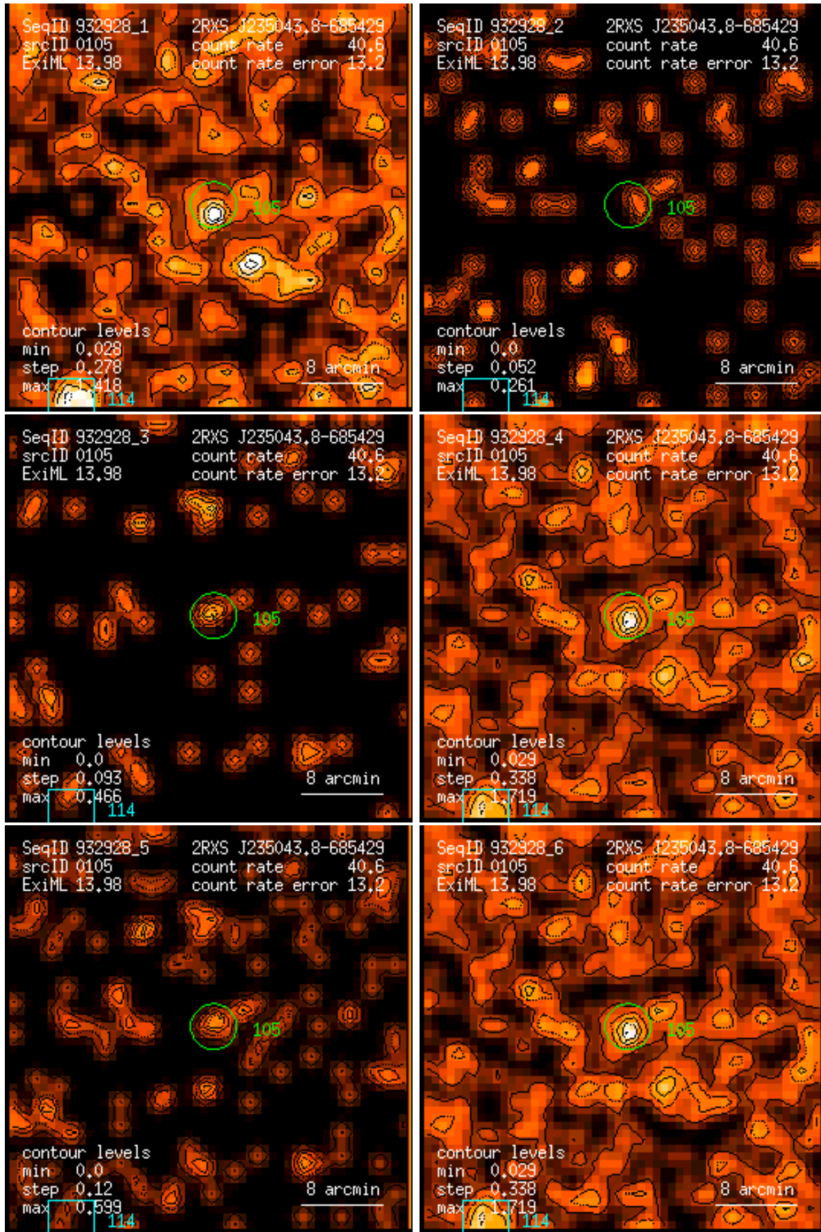
Figure 105: RASS 932928: detection 0105: band rate images, Gaussian filter: (1) PSPC channels 11 – 41, (2) 52 – 90, (3) 91 – 201, (4) 11 – 235, (5) 52 – 201, (6) 11 – 201. Broad band rates in counts/ks. Band rate contour levels in counts/ks/arcmin 2 .
