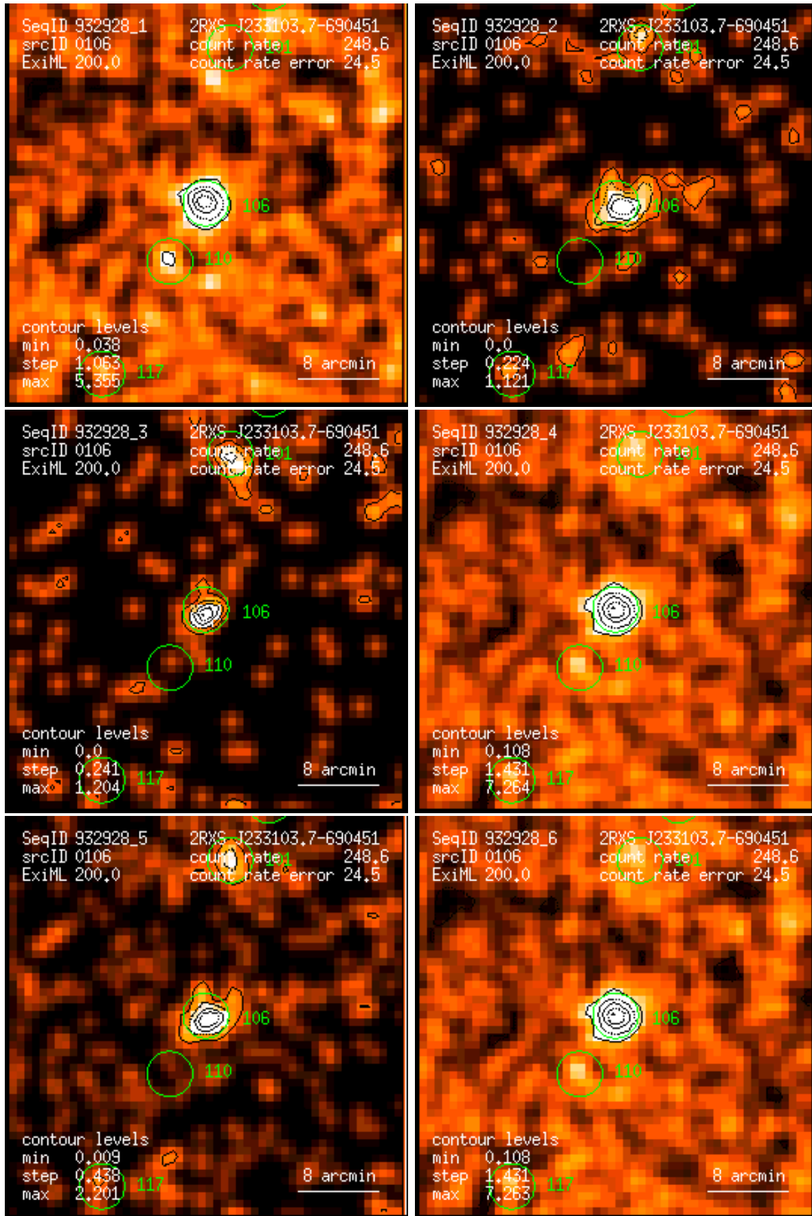
Figure 106: RASS 932928: detection 0106: band rate images, Gaussian filter: (1) PSPC channels 11 – 41, (2) 52 – 90, (3) 91 – 201, (4) 11 – 235, (5) 52 – 201, (6) 11 – 201. Broad band rates in counts/ks. Band rate contour levels in counts/ks/arcmin 2 .
