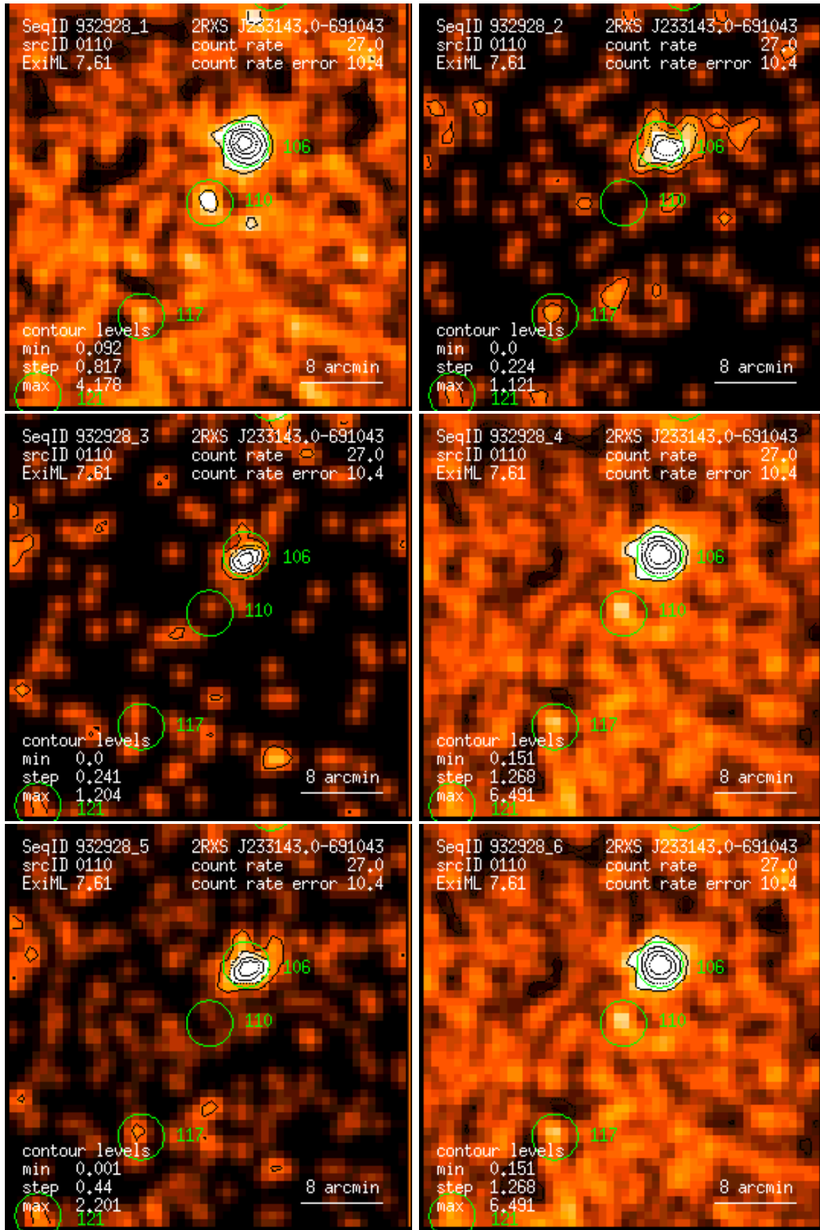
Figure 110: RASS 932928: detection 0110: band rate images, Gaussian filter: (1) PSPC channels 11 – 41, (2) 52 – 90, (3) 91 – 201, (4) 11 – 235, (5) 52 – 201, (6) 11 – 201. Broad band rates in counts/ks. Band rate contour levels in counts/ks/arcmin 2 .
