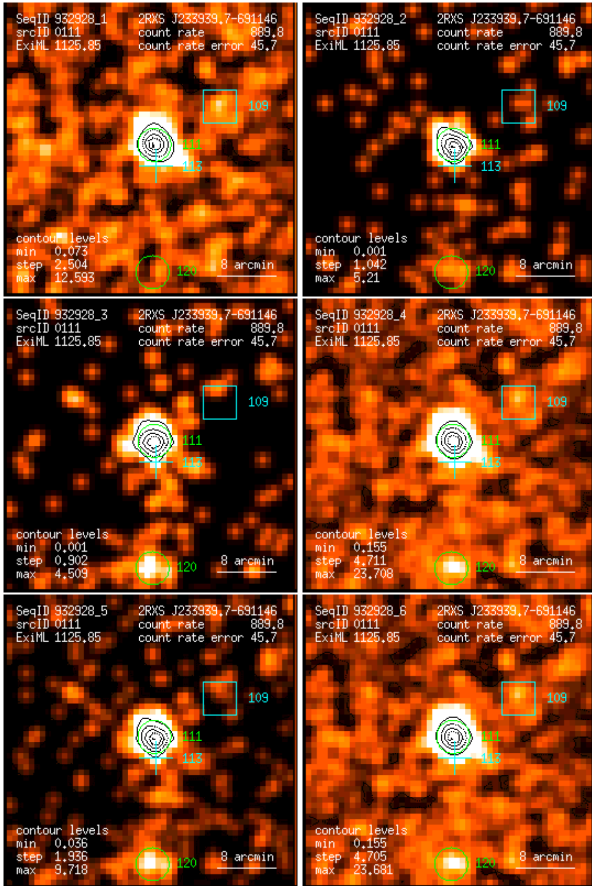
Figure 111: RASS 932928: detection 0111: band rate images, Gaussian filter: (1) PSPC channels 11 – 41, (2) 52 – 90, (3) 91 – 201, (4) 11 – 235, (5) 52 – 201, (6) 11 – 201. Broad band rates in counts/ks. Band rate contour levels in counts/ks/arcmin 2 .
