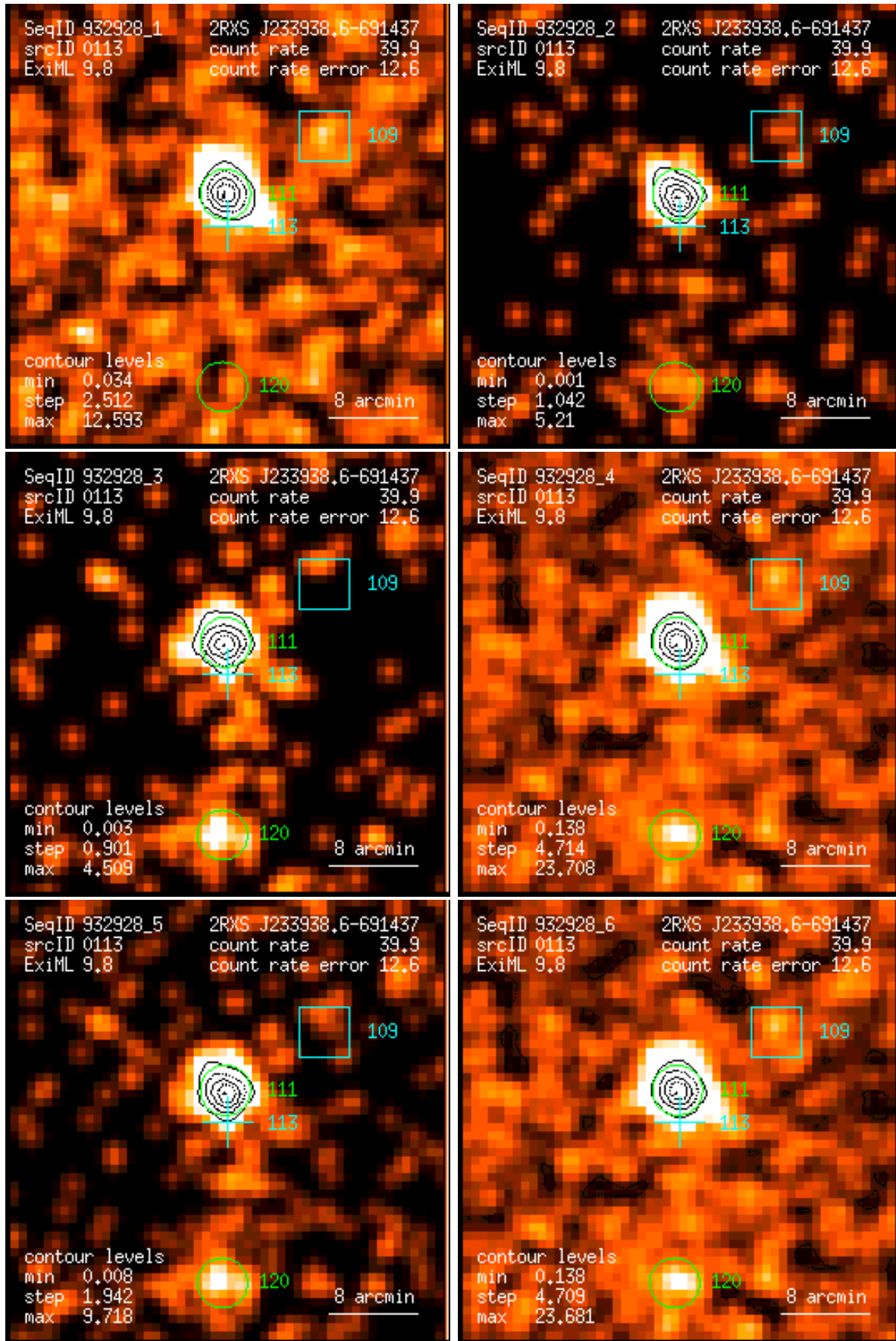
Figure 113: RASS 932928: detection 0113: band rate images, Gaussian filter: (1) PSPC channels 11 – 41, (2) 52 – 90, (3) 91 – 201, (4) 11 – 235, (5) 52 – 201, (6) 11 – 201. Broad band rates in counts/ks. Band rate contour levels in counts/ks/arcmin 2 .
