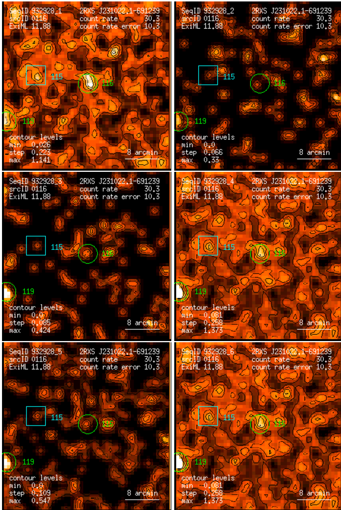
Figure 116: RASS 932928: detection 0116: band rate images, Gaussian filter: (1) PSPC channels 11 – 41, (2) 52 – 90, (3) 91 – 201, (4) 11 – 235, (5) 52 – 201, (6) 11 – 201. Broad band rates in counts/ks. Band rate contour levels in counts/ks/arcmin 2 .
