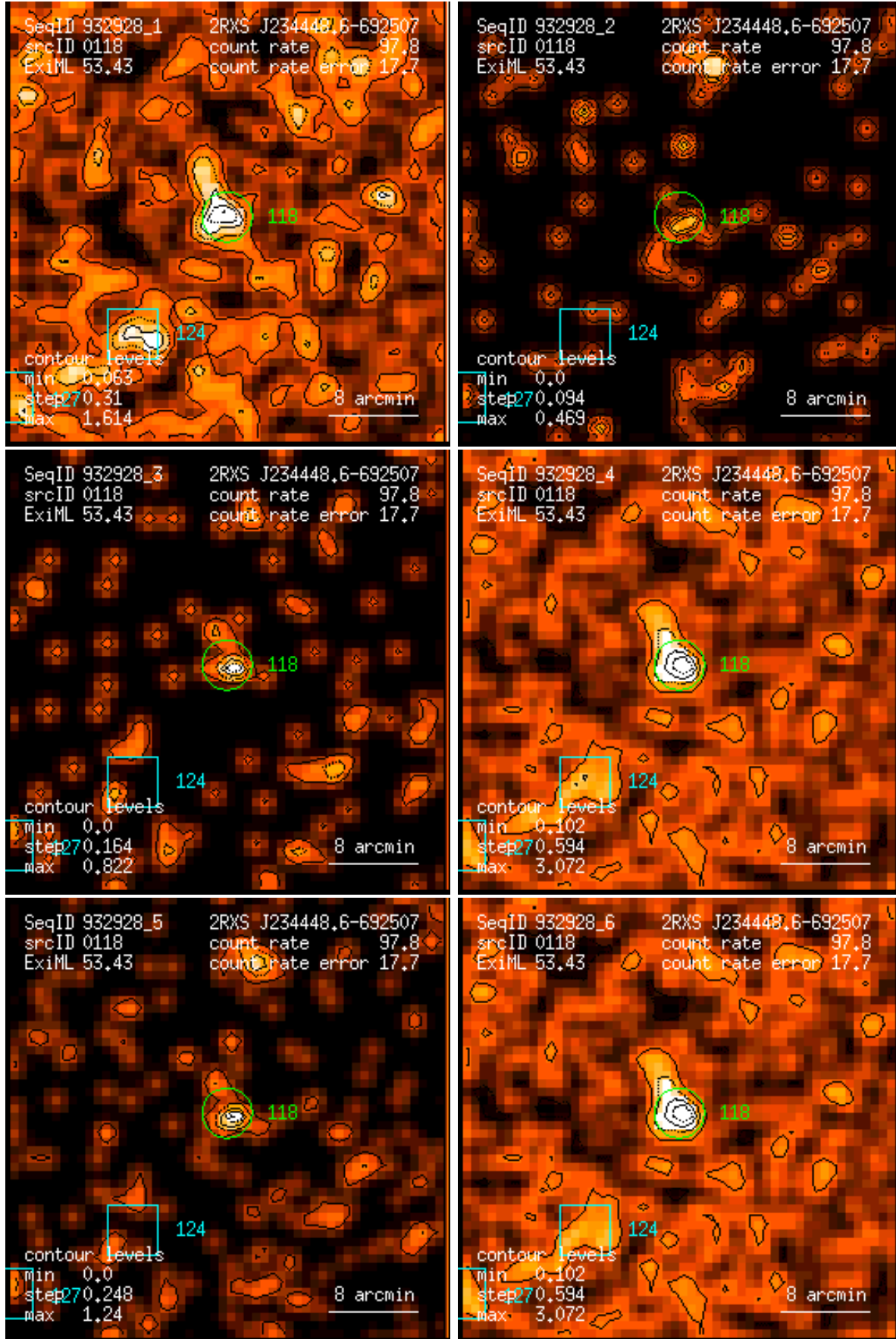
Figure 118: RASS 932928: detection 0118: band rate images, Gaussian filter: (1) PSPC channels 11 – 41, (2) 52 – 90, (3) 91 – 201, (4) 11 – 235, (5) 52 – 201, (6) 11 – 201. Broad band rates in counts/ks. Band rate contour levels in counts/ks/arcmin 2 .
