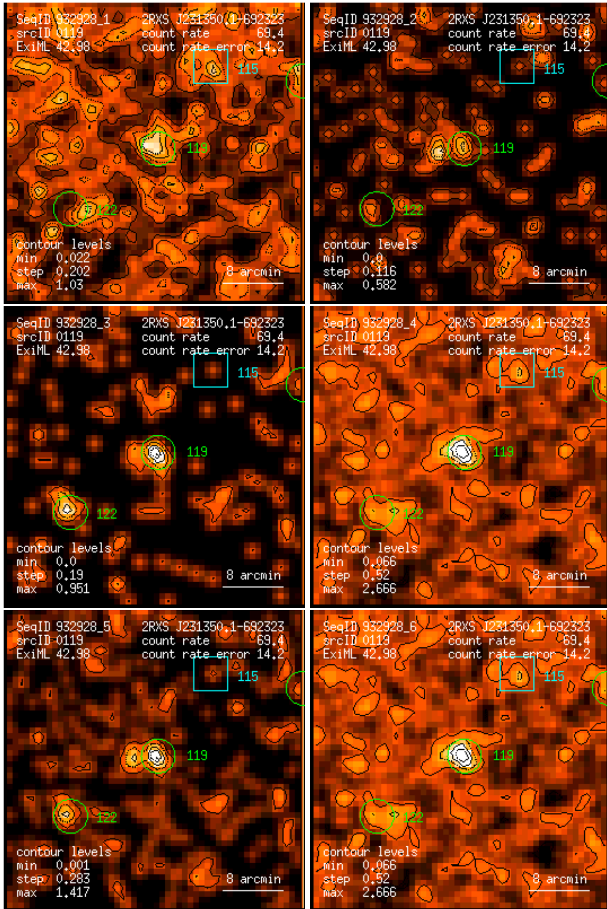
Figure 119: RASS 932928: detection 0119: band rate images, Gaussian filter: (1) PSPC channels 11 – 41, (2) 52 – 90, (3) 91 – 201, (4) 11 – 235, (5) 52 – 201, (6) 11 – 201. Broad band rates in counts/ks. Band rate contour levels in counts/ks/arcmin 2 .
