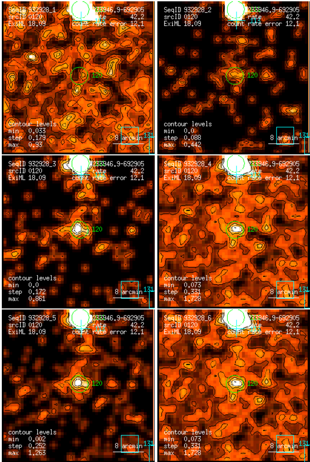
Figure 120: RASS 932928: detection 0120: band rate images, Gaussian filter: (1) PSPC channels 11 – 41, (2) 52 – 90, (3) 91 – 201, (4) 11 – 235, (5) 52 – 201, (6) 11 – 201. Broad band rates in counts/ks. Band rate contour levels in counts/ks/arcmin 2 .
