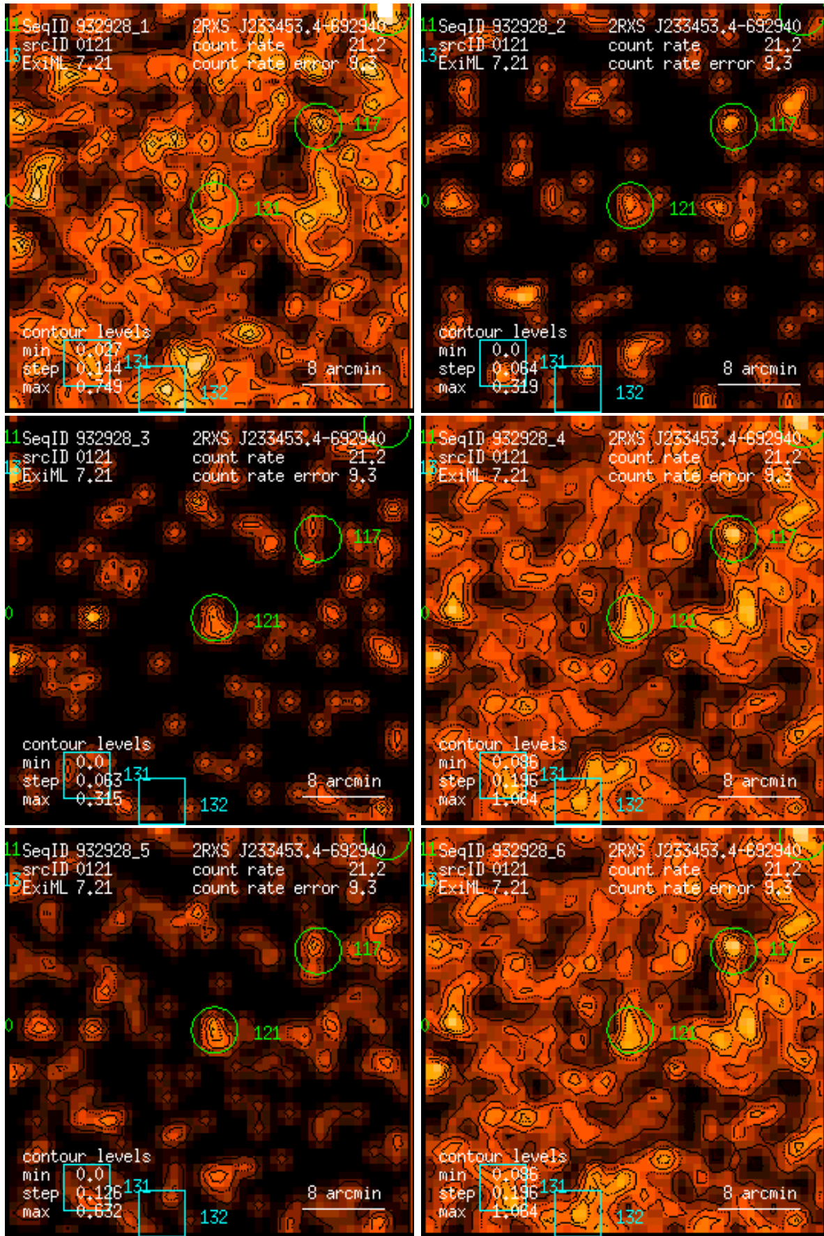
Figure 121: RASS 932928: detection 0121: band rate images, Gaussian filter: (1) PSPC channels 11 – 41, (2) 52 – 90, (3) 91 – 201, (4) 11 – 235, (5) 52 – 201, (6) 11 – 201. Broad band rates in counts/ks. Band rate contour levels in counts/ks/arcmin 2 .
