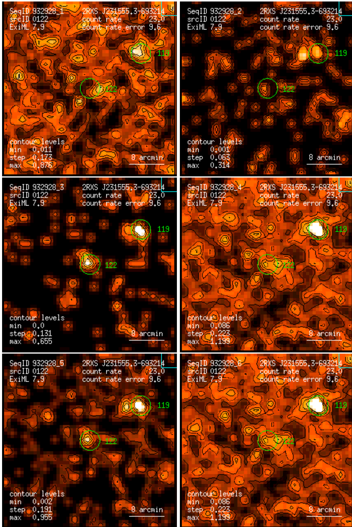
Figure 122: RASS 932928: detection 0122: band rate images, Gaussian filter: (1) PSPC channels 11 – 41, (2) 52 – 90, (3) 91 – 201, (4) 11 – 235, (5) 52 – 201, (6) 11 – 201. Broad band rates in counts/ks. Band rate contour levels in counts/ks/arcmin 2 .
