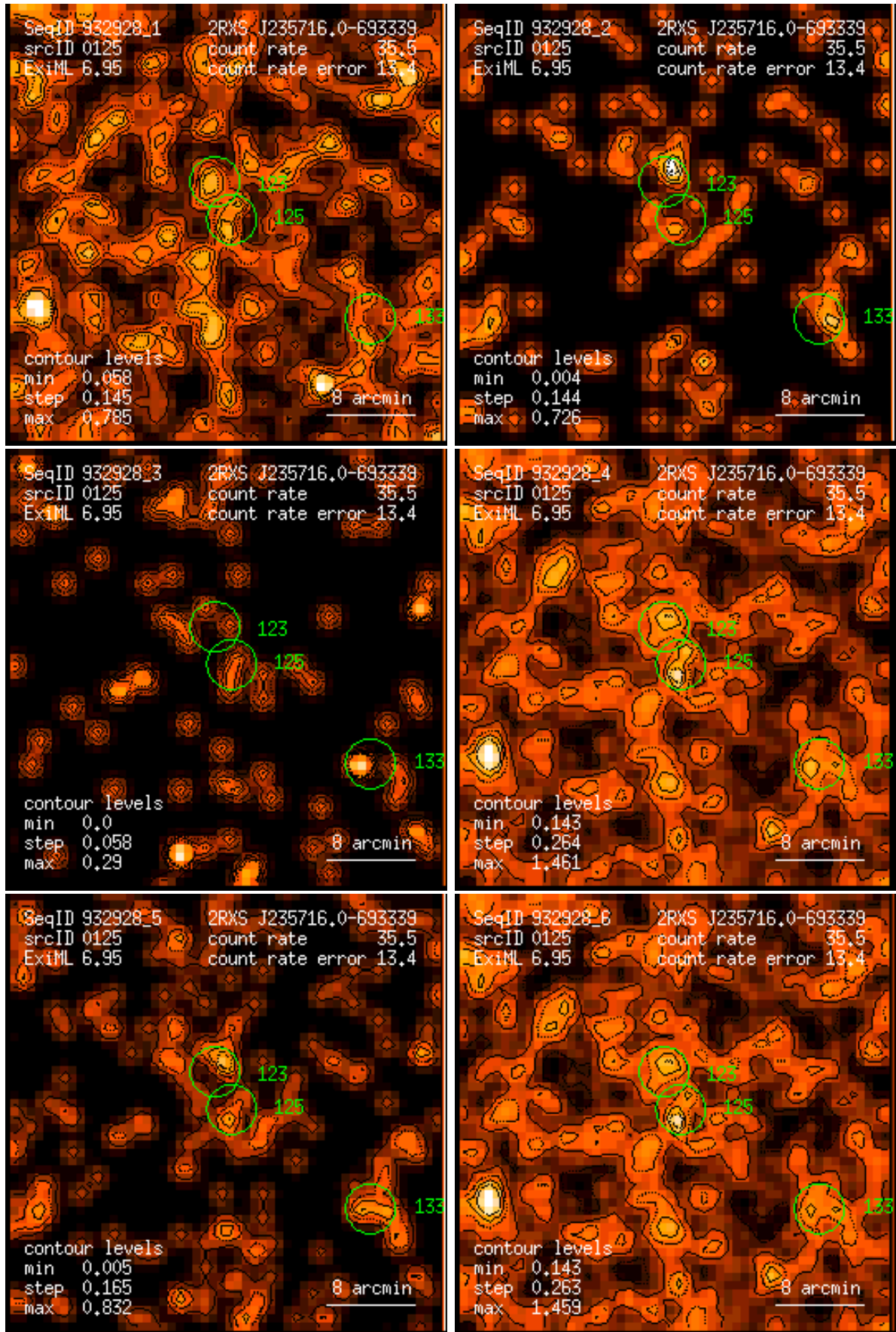
Figure 125: RASS 932928: detection 0125: band rate images, Gaussian filter: (1) PSPC channels 11 – 41, (2) 52 – 90, (3) 91 – 201, (4) 11 – 235, (5) 52 – 201, (6) 11 – 201. Broad band rates in counts/ks. Band rate contour levels in counts/ks/arcmin 2 .
