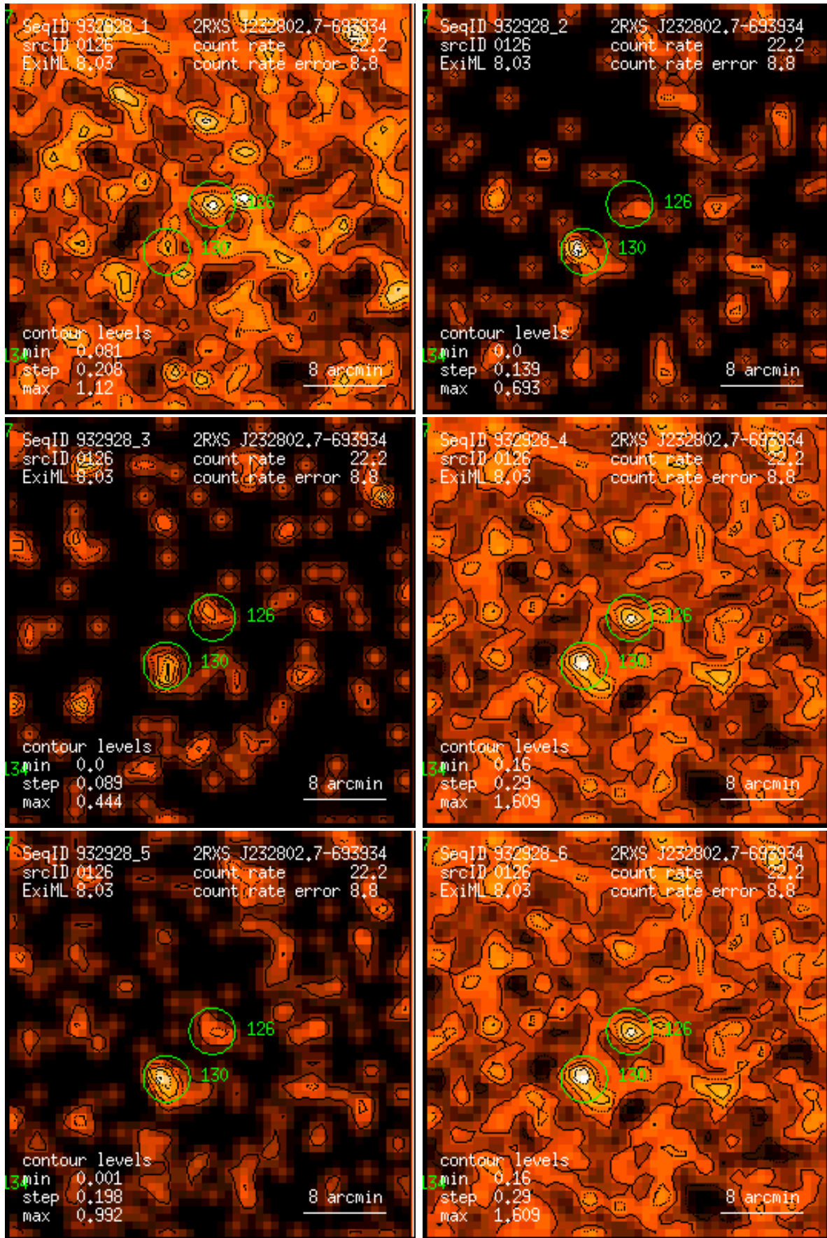
Figure 126: RASS 932928: detection 0126: band rate images, Gaussian filter: (1) PSPC channels 11 – 41, (2) 52 – 90, (3) 91 – 201, (4) 11 – 235, (5) 52 – 201, (6) 11 – 201. Broad band rates in counts/ks. Band rate contour levels in counts/ks/arcmin 2 .
