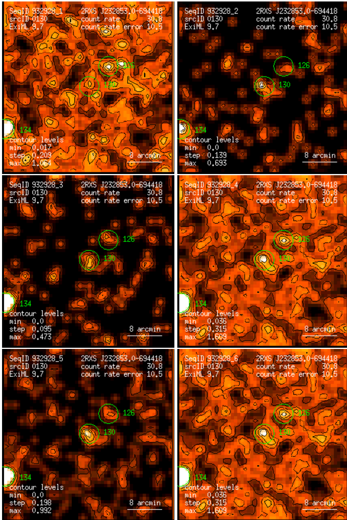
Figure 130: RASS 932928: detection 0130: band rate images, Gaussian filter: (1) PSPC channels 11 – 41, (2) 52 – 90, (3) 91 – 201, (4) 11 – 235, (5) 52 – 201, (6) 11 – 201. Broad band rates in counts/ks. Band rate contour levels in counts/ks/arcmin 2 .
