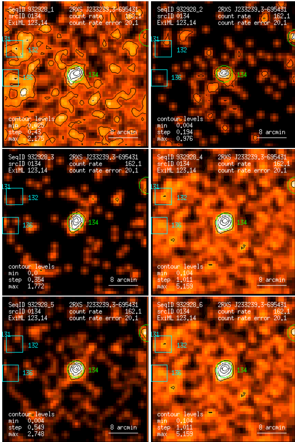
Figure 134: RASS 932928: detection 0134: band rate images, Gaussian filter: (1) PSPC channels 11 – 41, (2) 52 – 90, (3) 91 – 201, (4) 11 – 235, (5) 52 – 201, (6) 11 – 201. Broad band rates in counts/ks. Band rate contour levels in counts/ks/arcmin 2 .
