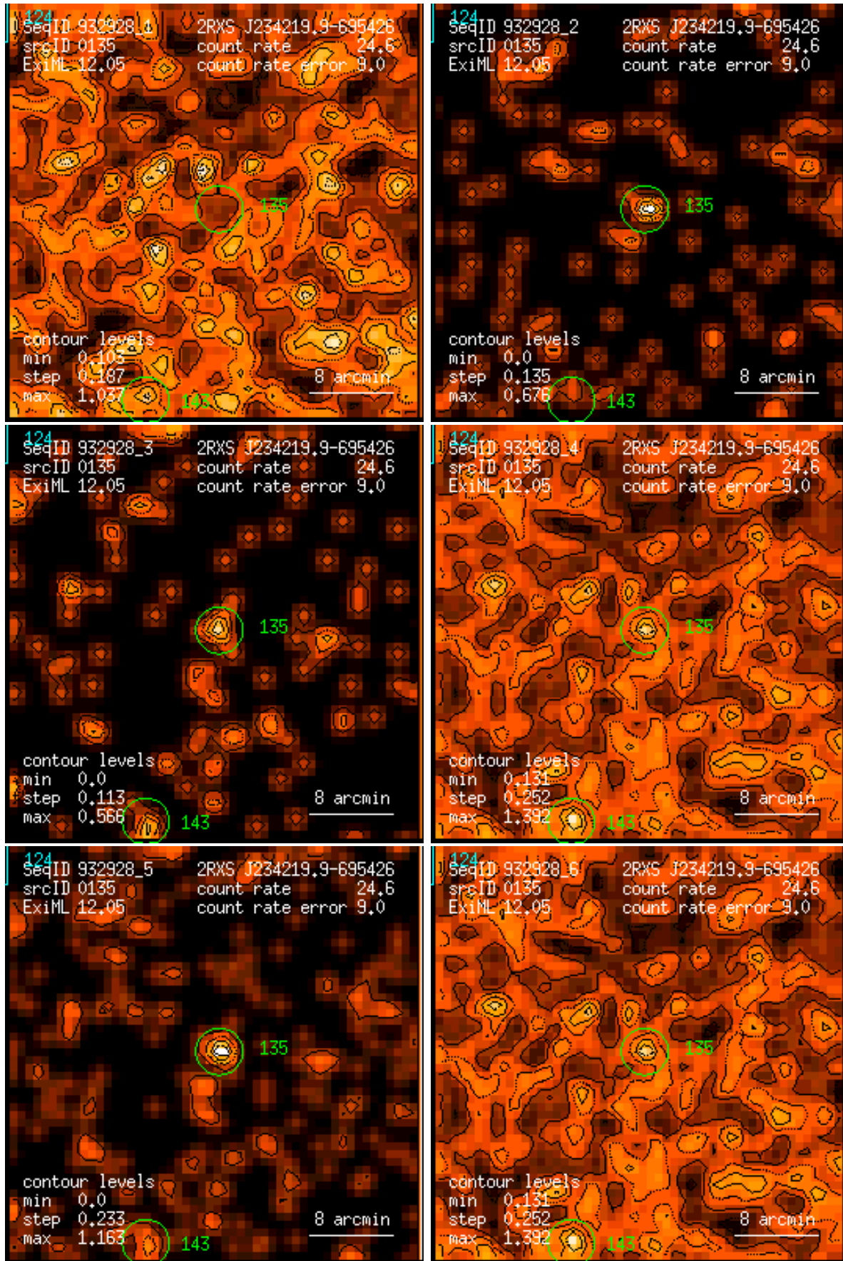
Figure 135: RASS 932928: detection 0135: band rate images, Gaussian filter: (1) PSPC channels 11 – 41, (2) 52 – 90, (3) 91 – 201, (4) 11 – 235, (5) 52 – 201, (6) 11 – 201. Broad band rates in counts/ks. Band rate contour levels in counts/ks/arcmin 2 .
